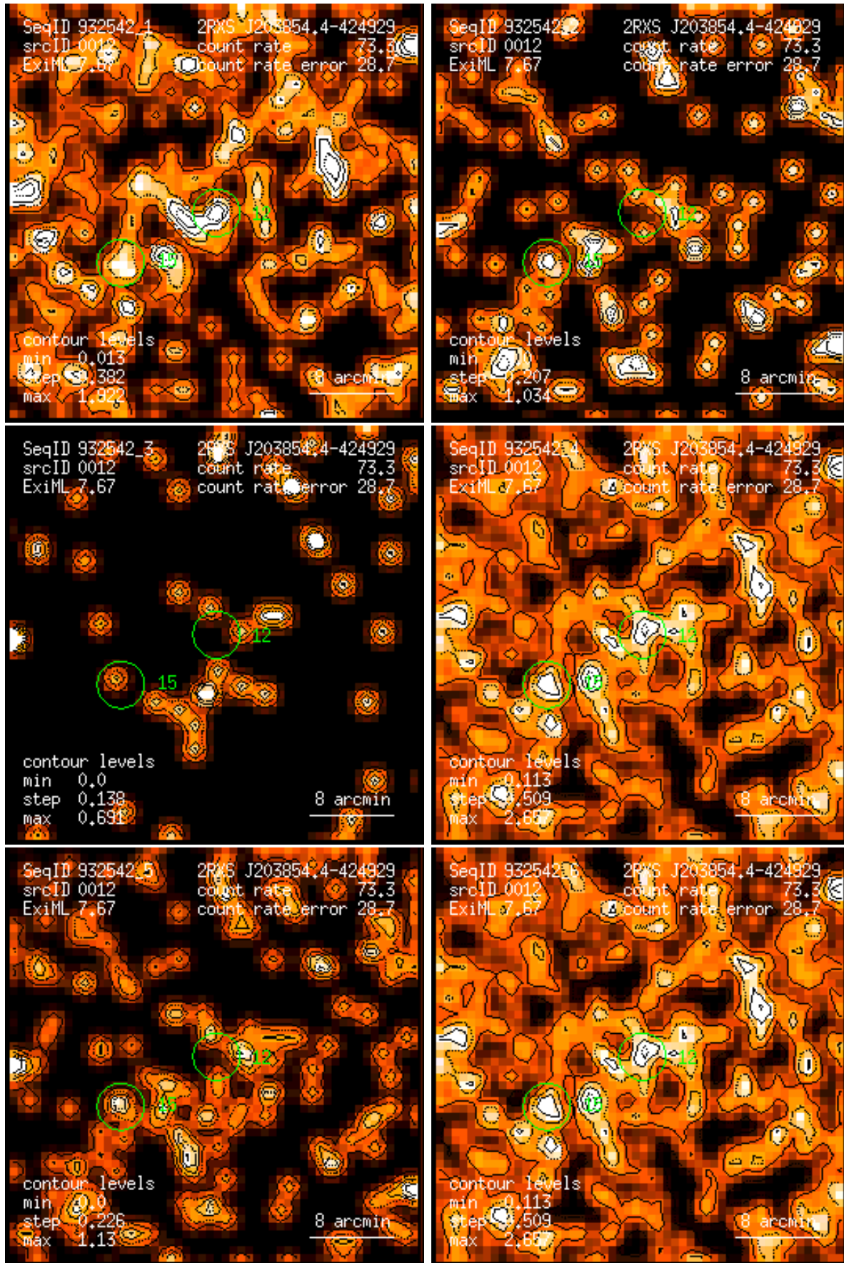
Figure 12: RASS 932542: detection 0012: band rate images, Gaussian filter: (1) PSPC channels 11 – 41, (2) 52 – 90, (3) 91 – 201, (4) 11 – 235, (5) 52 – 201, (6) 11 – 201. Broad band rates in counts/ks. Band rate contour levels in counts/ks/arcmin 2 .
