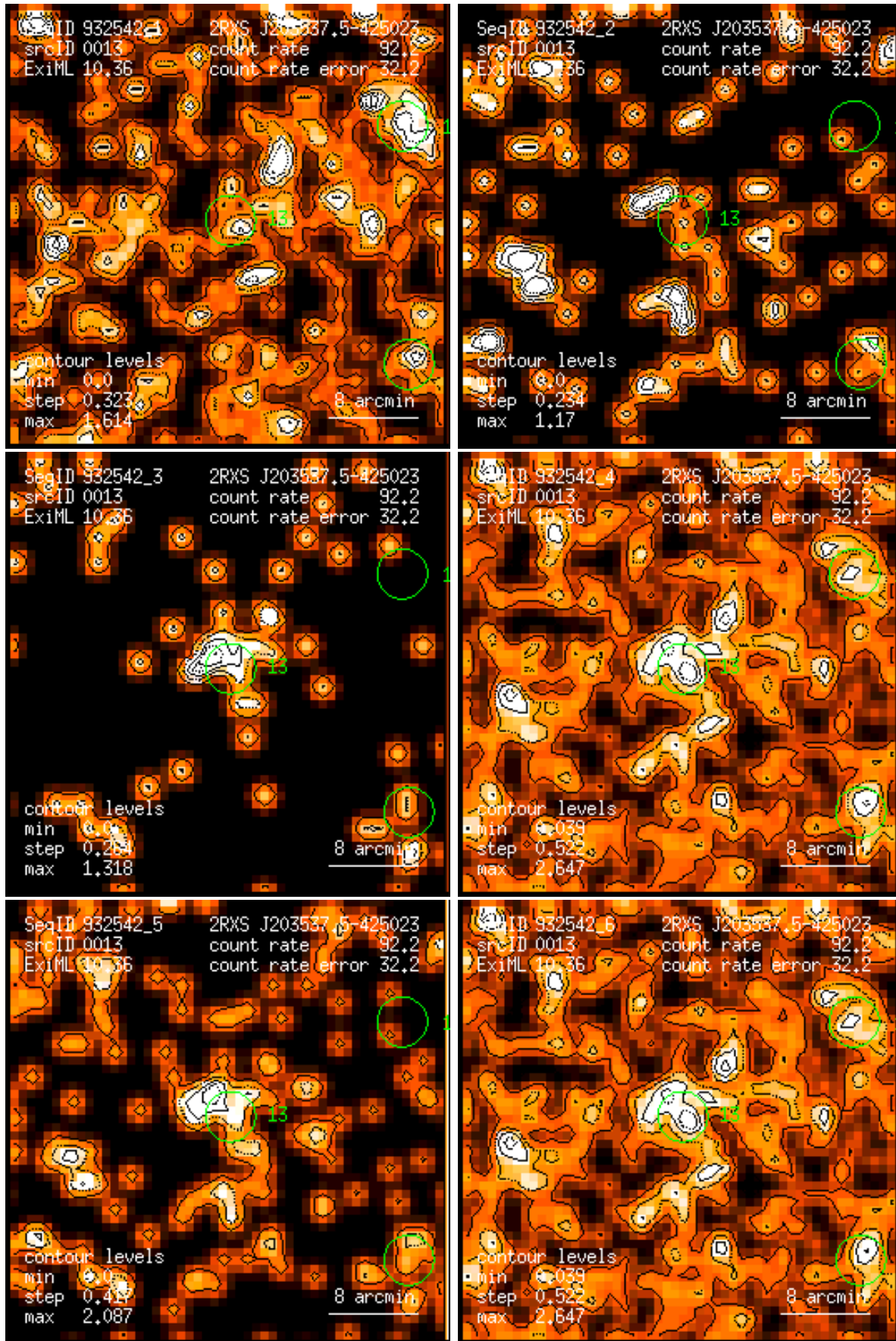
Figure 13: RASS 932542: detection 0013: band rate images, Gaussian filter: (1) PSPC channels 11 – 41, (2) 52 – 90, (3) 91 – 201, (4) 11 – 235, (5) 52 – 201, (6) 11 – 201. Broad band rates in counts/ks. Band rate contour levels in counts/ks/arcmin 2 .
