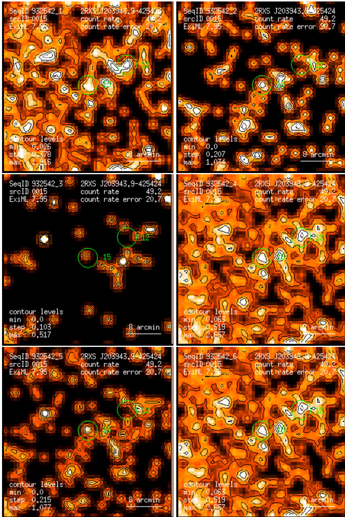
Figure 15: RASS 932542: detection 0015: band rate images, Gaussian filter: (1) PSPC channels 11 – 41, (2) 52 – 90, (3) 91 – 201, (4) 11 – 235, (5) 52 – 201, (6) 11 – 201. Broad band rates in counts/ks. Band rate contour levels in counts/ks/arcmin 2 .
