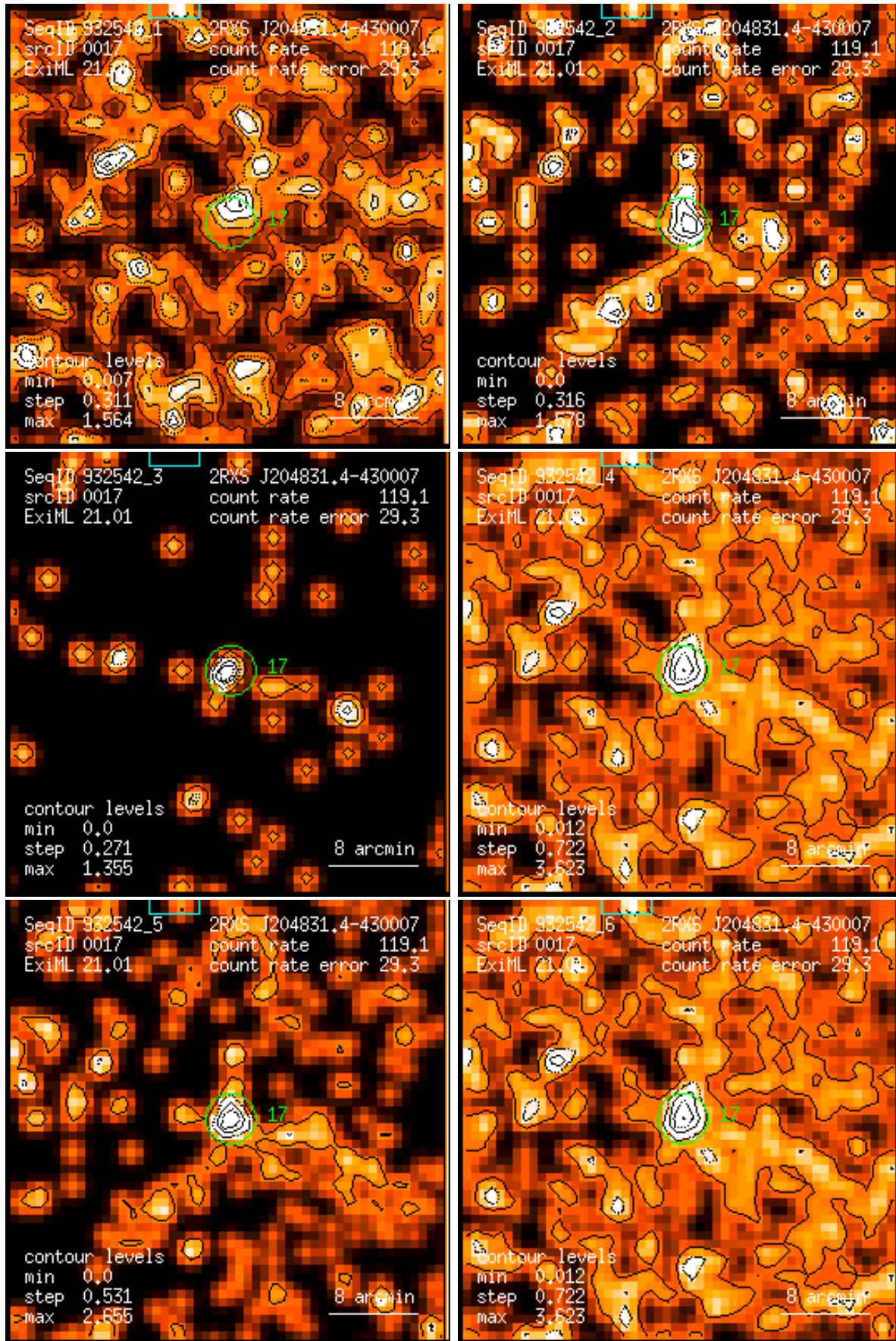
Figure 17: RASS 932542: detection 0017: band rate images, Gaussian filter: (1) PSPC channels 11 – 41, (2) 52 – 90, (3) 91 – 201, (4) 11 – 235, (5) 52 – 201, (6) 11 – 201. Broad band rates in counts/ks. Band rate contour levels in counts/ks/arcmin 2 .
