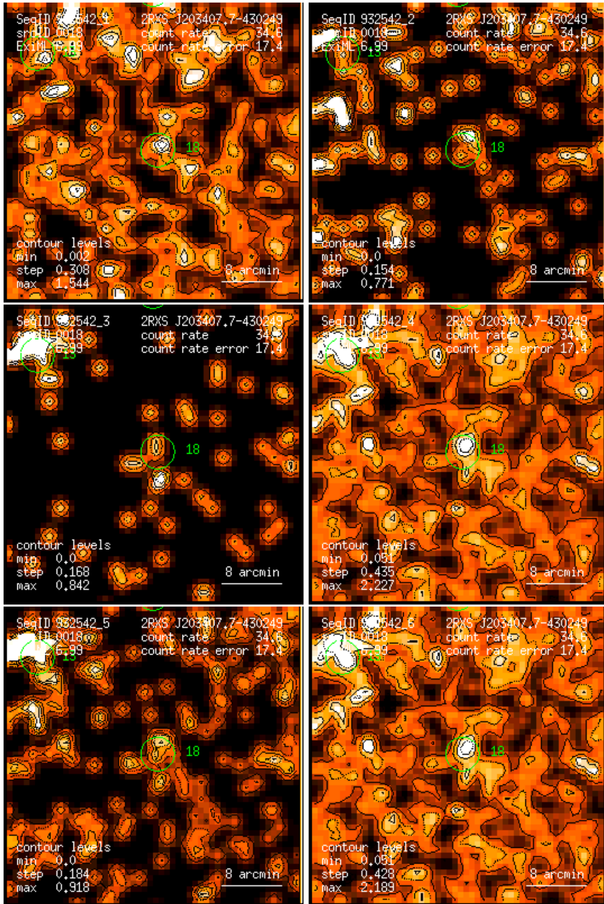
Figure 18: RASS 932542: detection 0018: band rate images, Gaussian filter: (1) PSPC channels 11 – 41, (2) 52 – 90, (3) 91 – 201, (4) 11 – 235, (5) 52 – 201, (6) 11 – 201. Broad band rates in counts/ks. Band rate contour levels in counts/ks/arcmin 2 .
