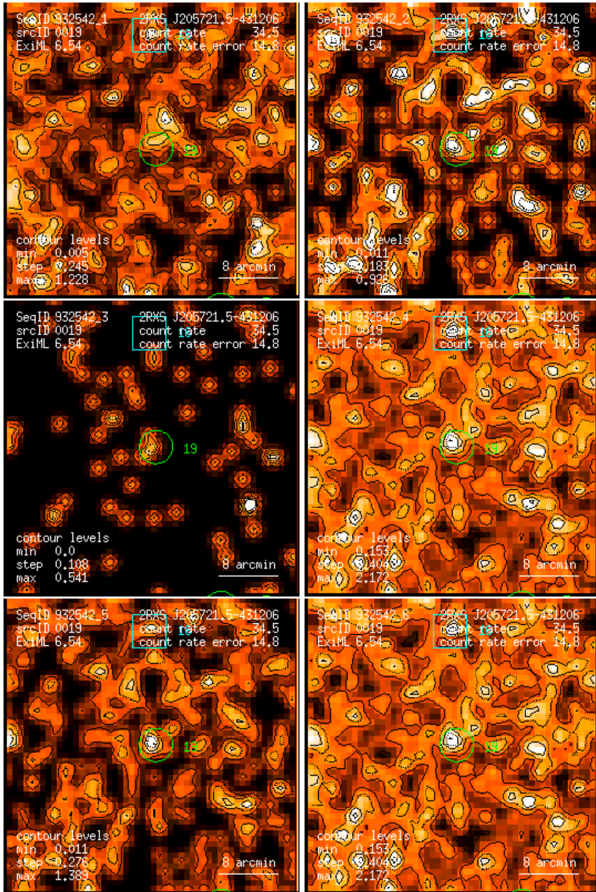
Figure 19: RASS 932542: detection 0019: band rate images, Gaussian filter: (1) PSPC channels 11 – 41, (2) 52 – 90, (3) 91 – 201, (4) 11 – 235, (5) 52 – 201, (6) 11 – 201. Broad band rates in counts/ks. Band rate contour levels in counts/ks/arcmin 2 .
