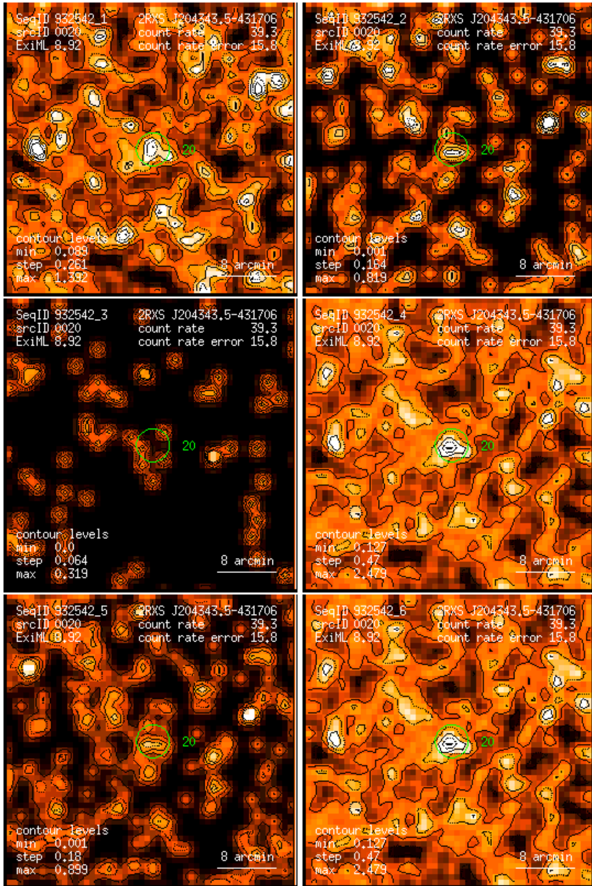
Figure 20: RASS 932542: detection 0020: band rate images, Gaussian filter: (1) PSPC channels 11 – 41, (2) 52 – 90, (3) 91 – 201, (4) 11 – 235, (5) 52 – 201, (6) 11 – 201. Broad band rates in counts/ks. Band rate contour levels in counts/ks/arcmin 2 .
