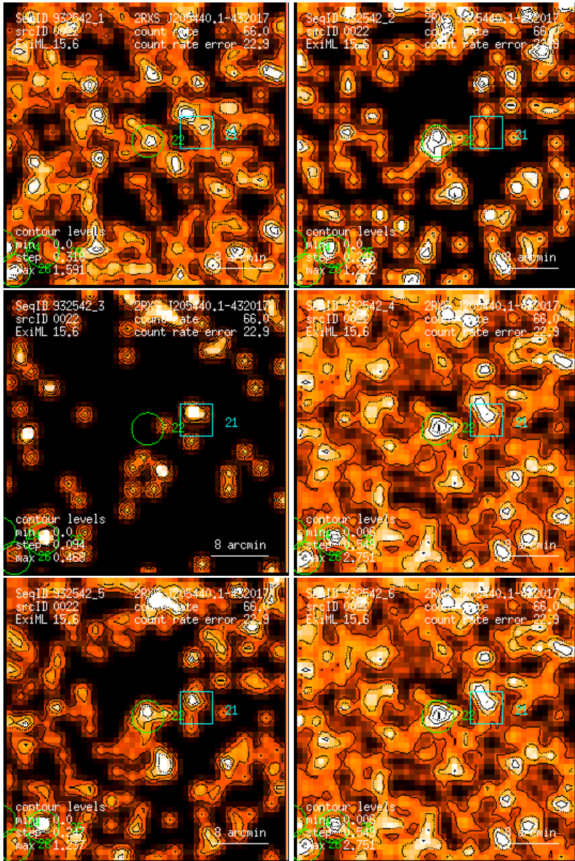
Figure 22: RASS 932542: detection 0022: band rate images, Gaussian filter: (1) PSPC channels 11 – 41, (2) 52 – 90, (3) 91 – 201, (4) 11 – 235, (5) 52 – 201, (6) 11 – 201. Broad band rates in counts/ks. Band rate contour levels in counts/ks/arcmin 2 .
