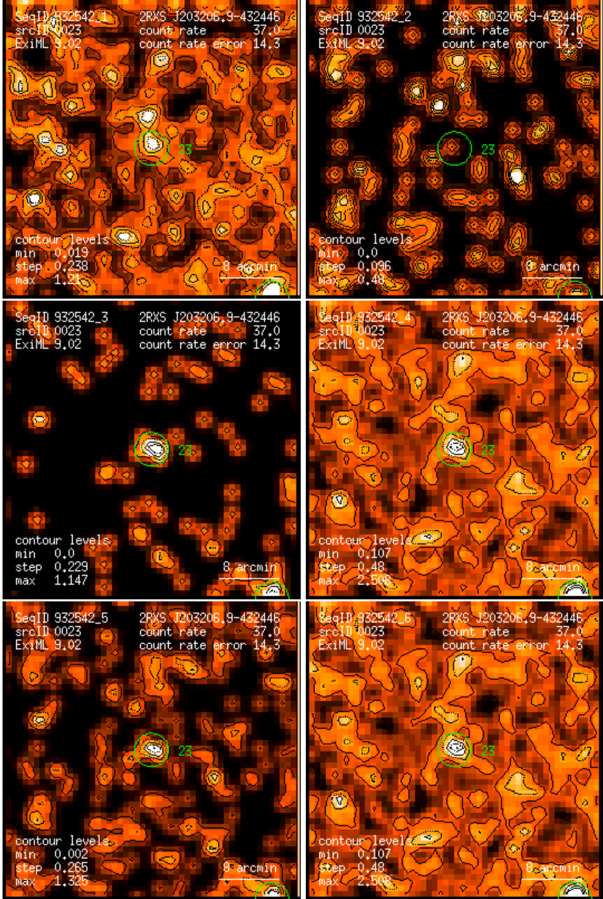
Figure 23: RASS 932542: detection 0023: band rate images, Gaussian filter: (1) PSPC channels 11 – 41, (2) 52 – 90, (3) 91 – 201, (4) 11 – 235, (5) 52 – 201, (6) 11 – 201. Broad band rates in counts/ks. Band rate contour levels in counts/ks/arcmin 2 .
