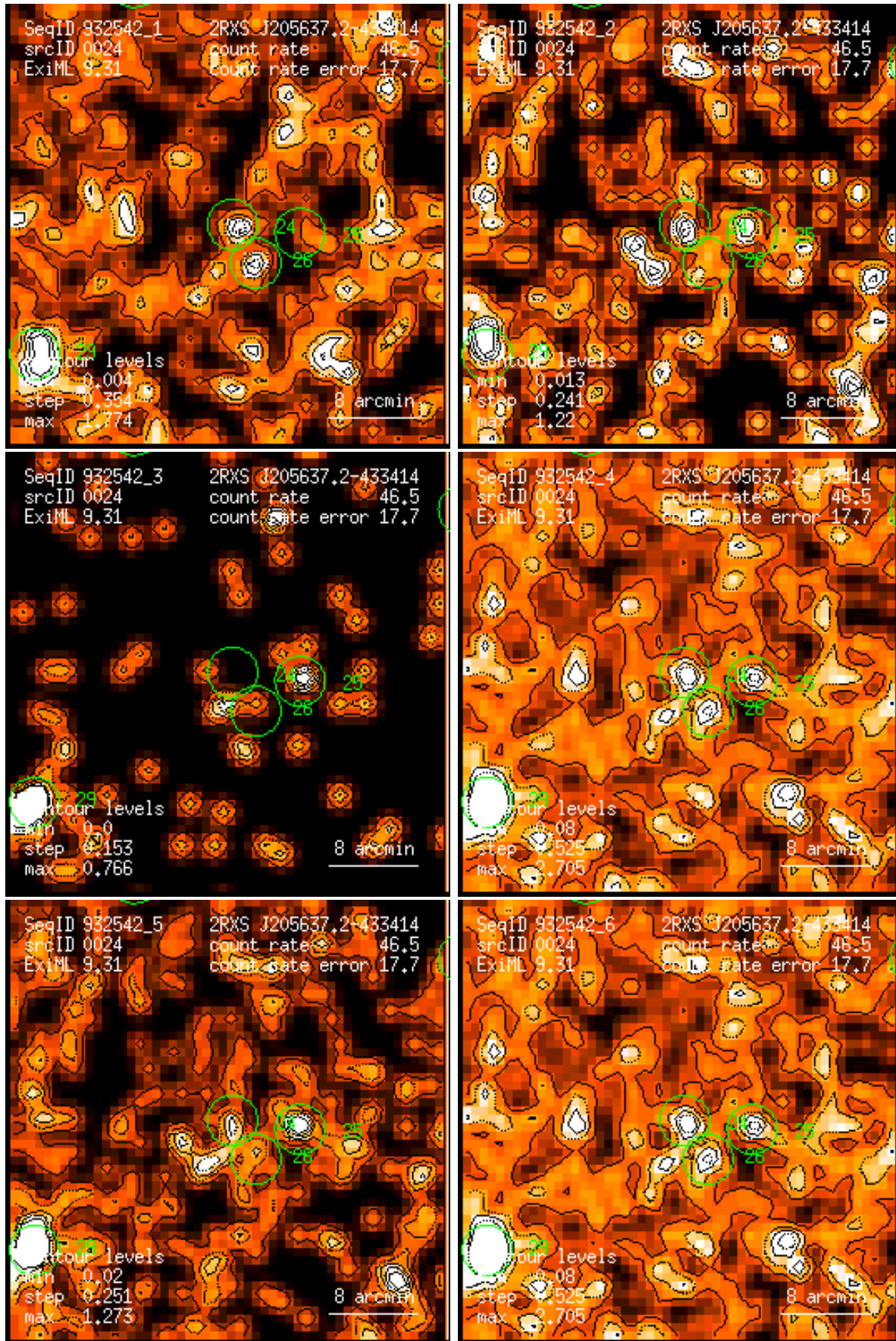
Figure 24: RASS 932542: detection 0024: band rate images, Gaussian filter: (1) PSPC channels 11 – 41, (2) 52 – 90, (3) 91 – 201, (4) 11 – 235, (5) 52 – 201, (6) 11 – 201. Broad band rates in counts/ks. Band rate contour levels in counts/ks/arcmin 2 .
