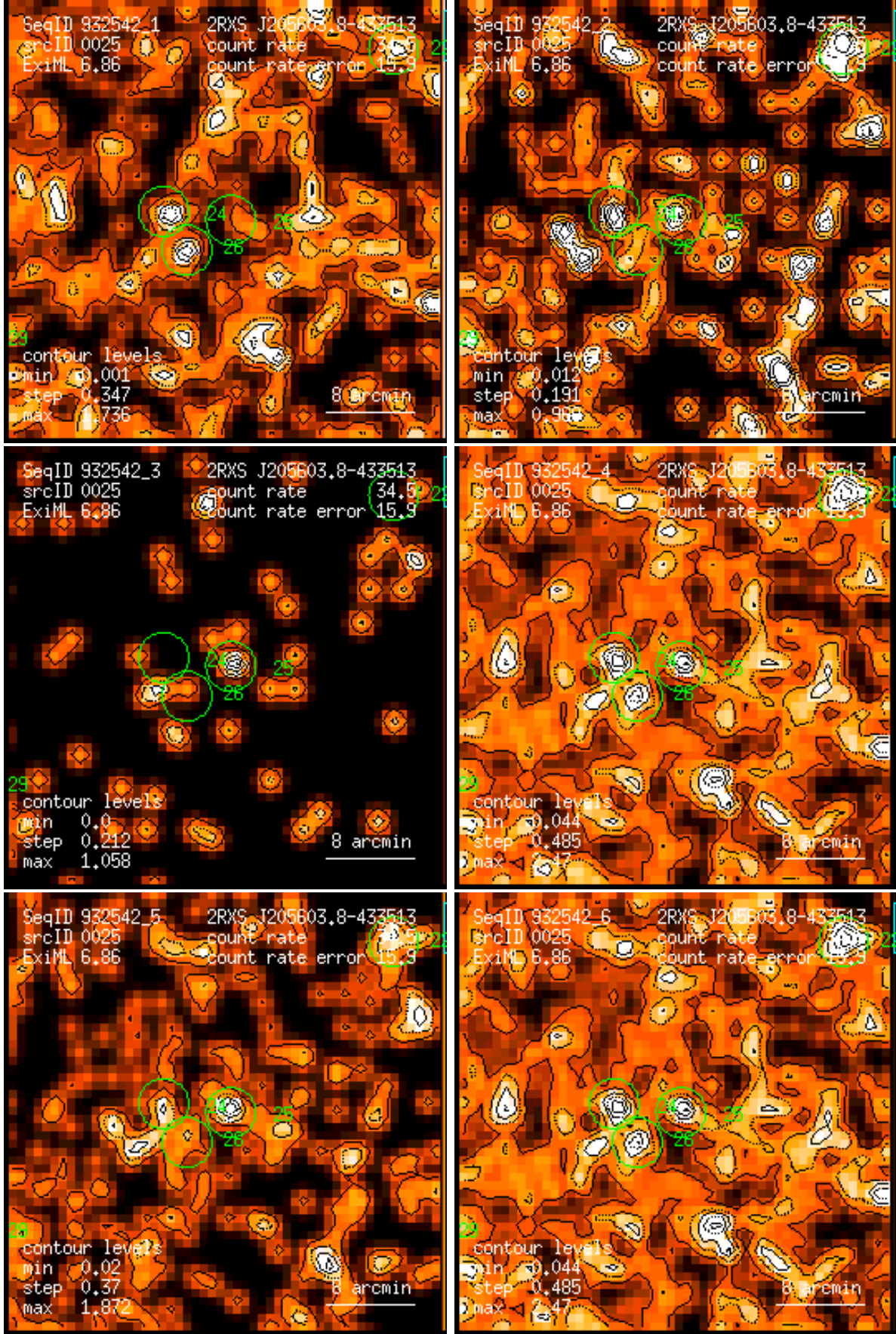
Figure 25: RASS 932542: detection 0025: band rate images, Gaussian filter: (1) PSPC channels 11 – 41, (2) 52 – 90, (3) 91 – 201, (4) 11 – 235, (5) 52 – 201, (6) 11 – 201. Broad band rates in counts/ks. Band rate contour levels in counts/ks/arcmin 2 .
