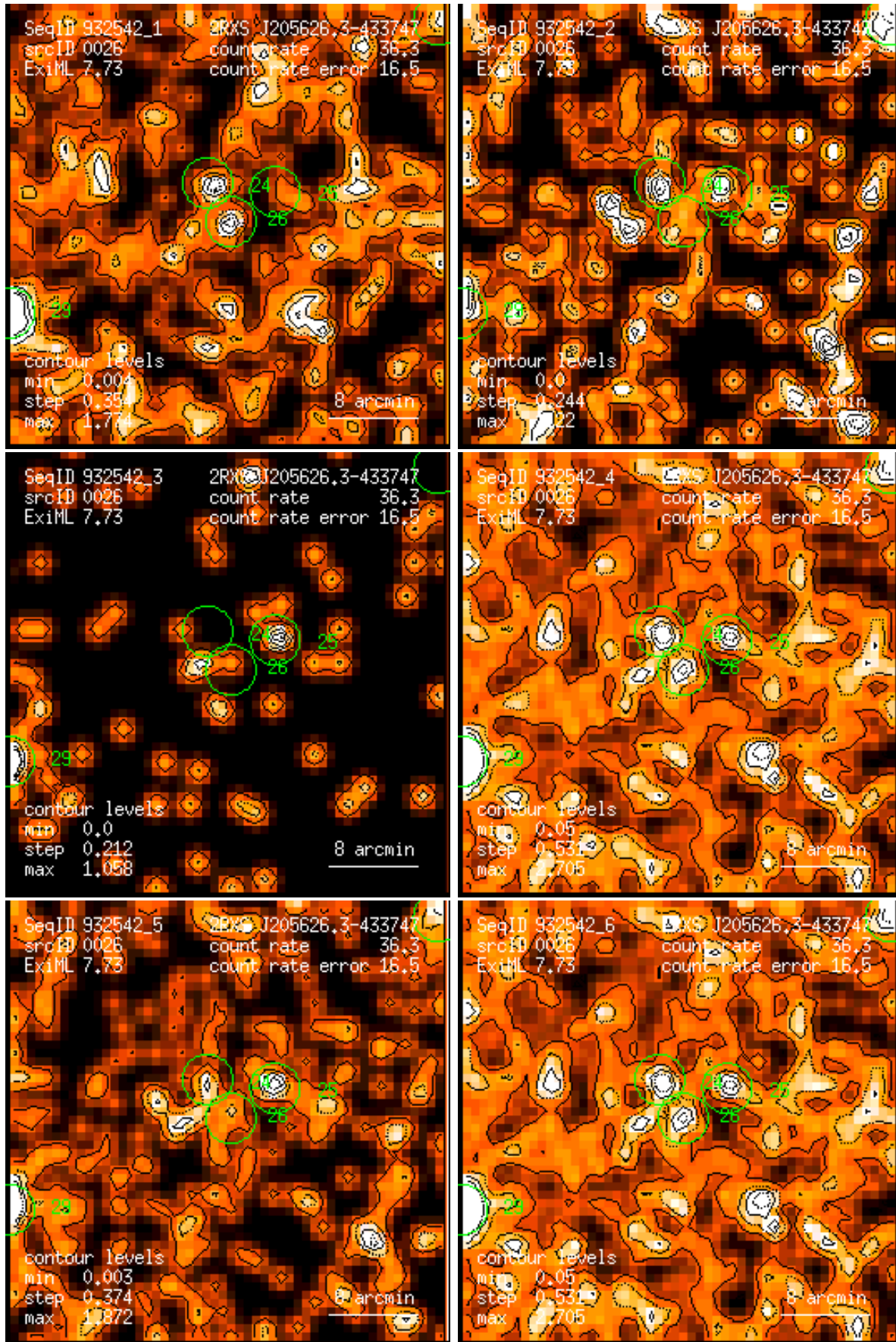
Figure 26: RASS 932542: detection 0026: band rate images, Gaussian filter: (1) PSPC channels 11 – 41, (2) 52 – 90, (3) 91 – 201, (4) 11 – 235, (5) 52 – 201, (6) 11 – 201. Broad band rates in counts/ks. Band rate contour levels in counts/ks/arcmin 2 .
