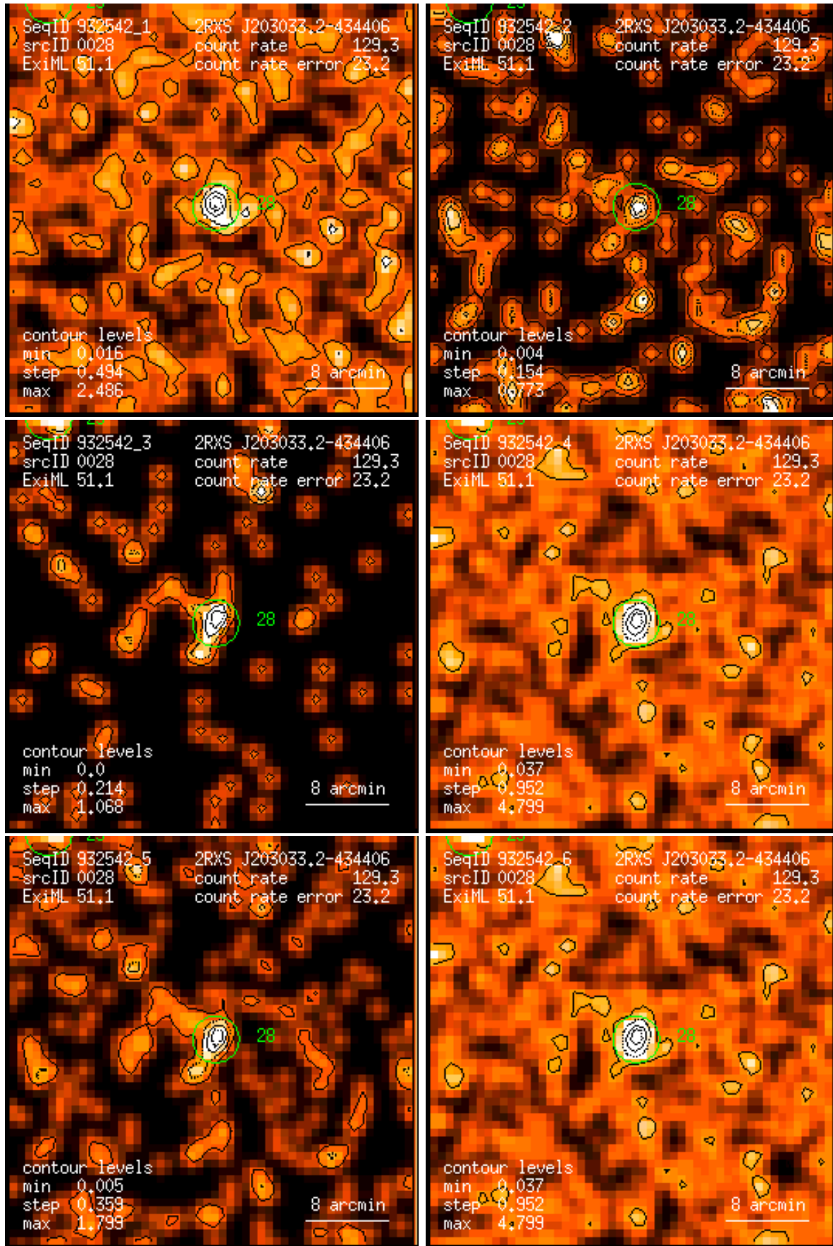
Figure 28: RASS 932542: detection 0028: band rate images, Gaussian filter: (1) PSPC channels 11 – 41, (2) 52 – 90, (3) 91 – 201, (4) 11 – 235, (5) 52 – 201, (6) 11 – 201. Broad band rates in counts/ks. Band rate contour levels in counts/ks/arcmin 2 .
