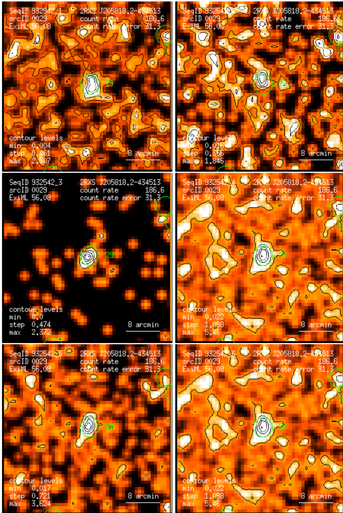
Figure 29: RASS 932542: detection 0029: band rate images, Gaussian filter: (1) PSPC channels 11 – 41, (2) 52 – 90, (3) 91 – 201, (4) 11 – 235, (5) 52 – 201, (6) 11 – 201. Broad band rates in counts/ks. Band rate contour levels in counts/ks/arcmin 2 .
