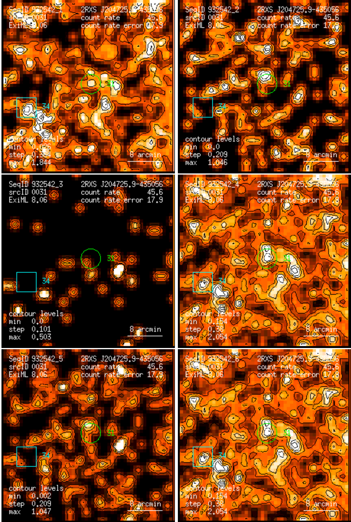
Figure 31: RASS 932542: detection 0031: band rate images, Gaussian filter: (1) PSPC channels 11 – 41, (2) 52 – 90, (3) 91 – 201, (4) 11 – 235, (5) 52 – 201, (6) 11 – 201. Broad band rates in counts/ks. Band rate contour levels in counts/ks/arcmin 2 .
