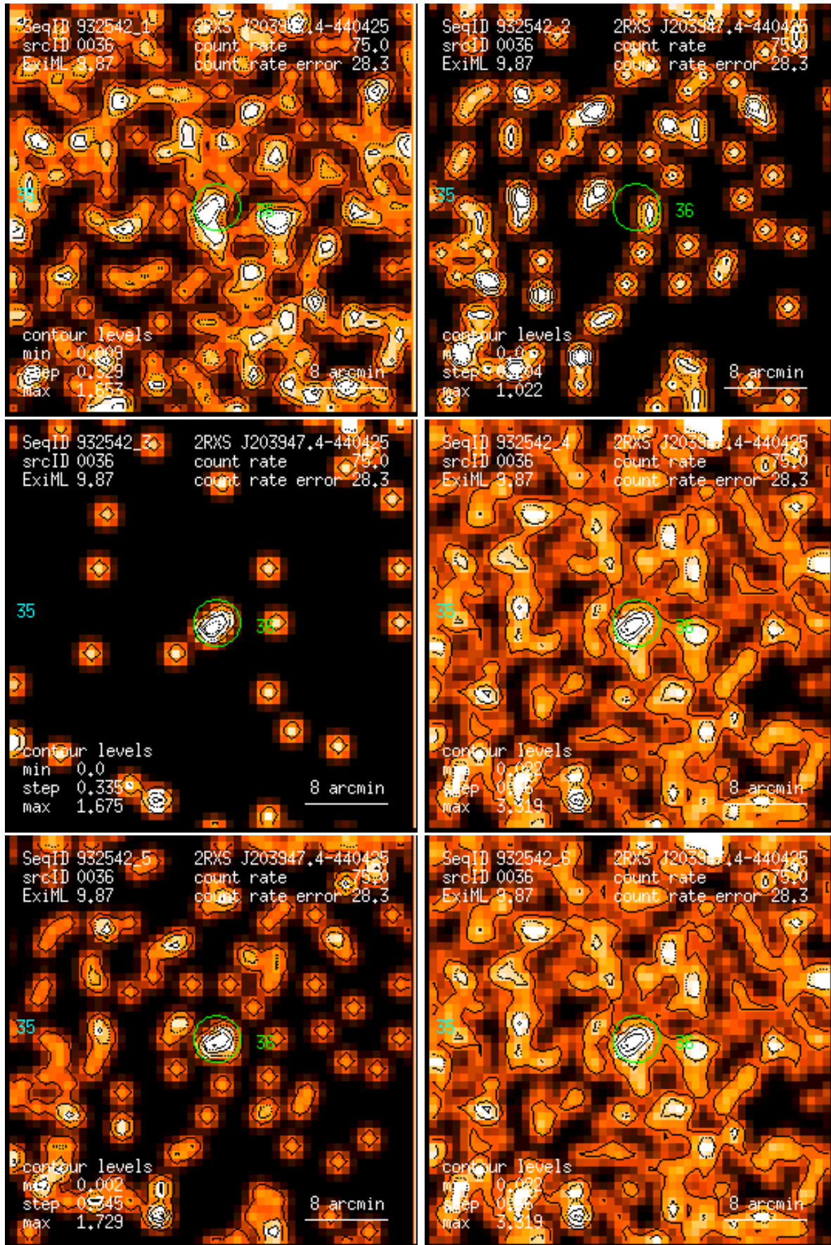
Figure 36: RASS 932542: detection 0036: band rate images, Gaussian filter: (1) PSPC channels 11 – 41, (2) 52 – 90, (3) 91 – 201, (4) 11 – 235, (5) 52 – 201, (6) 11 – 201. Broad band rates in counts/ks. Band rate contour levels in counts/ks/arcmin 2 .
