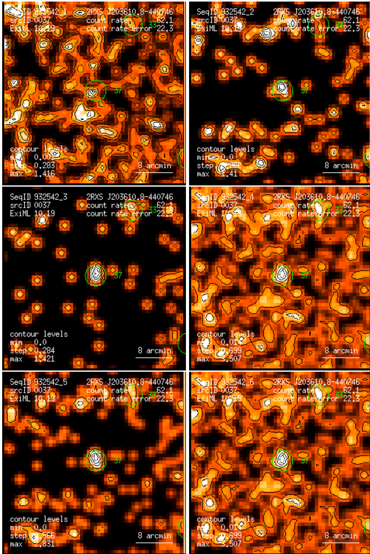
Figure 37: RASS 932542: detection 0037: band rate images, Gaussian filter: (1) PSPC channels 11 – 41, (2) 52 – 90, (3) 91 – 201, (4) 11 – 235, (5) 52 – 201, (6) 11 – 201. Broad band rates in counts/ks. Band rate contour levels in counts/ks/arcmin 2 .
