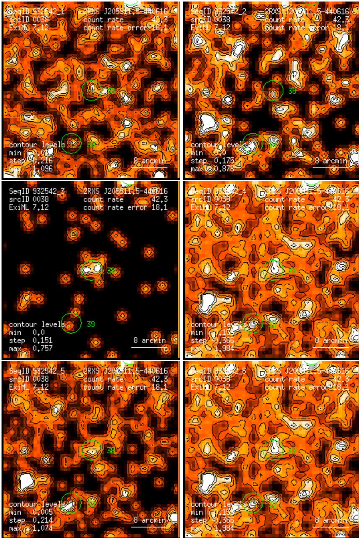
Figure 38: RASS 932542: detection 0038: band rate images, Gaussian filter: (1) PSPC channels 11 – 41, (2) 52 – 90, (3) 91 – 201, (4) 11 – 235, (5) 52 – 201, (6) 11 – 201. Broad band rates in counts/ks. Band rate contour levels in counts/ks/arcmin 2 .
