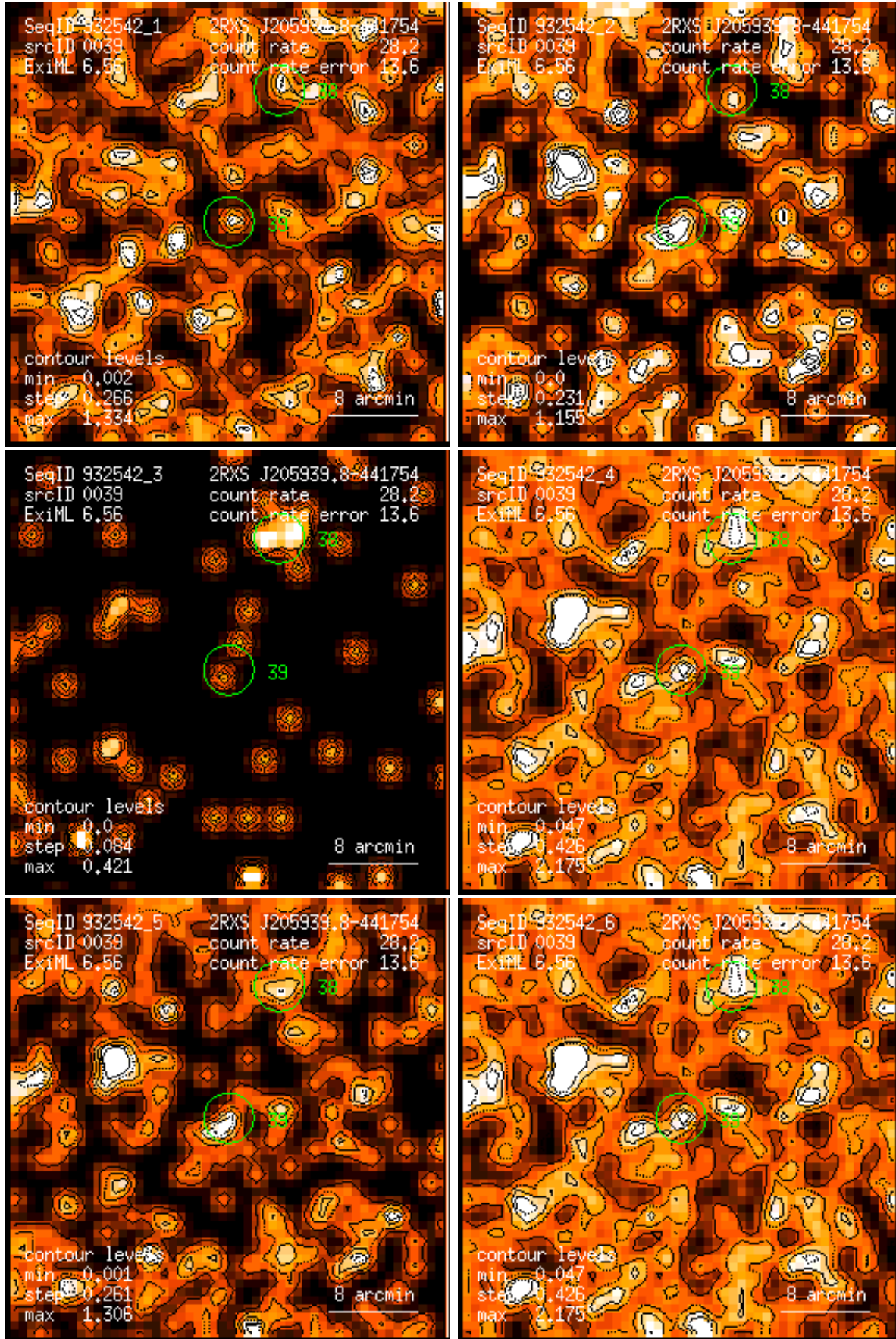
Figure 39: RASS 932542: detection 0039: band rate images, Gaussian filter: (1) PSPC channels 11 – 41, (2) 52 – 90, (3) 91 – 201, (4) 11 – 235, (5) 52 – 201, (6) 11 – 201. Broad band rates in counts/ks. Band rate contour levels in counts/ks/arcmin 2 .
