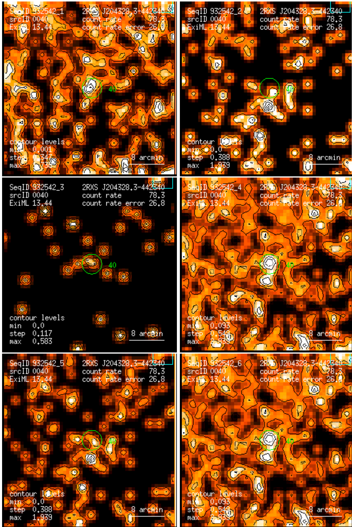
Figure 40: RASS 932542: detection 0040: band rate images, Gaussian filter: (1) PSPC channels 11 – 41, (2) 52 – 90, (3) 91 – 201, (4) 11 – 235, (5) 52 – 201, (6) 11 – 201. Broad band rates in counts/ks. Band rate contour levels in counts/ks/arcmin 2 .
