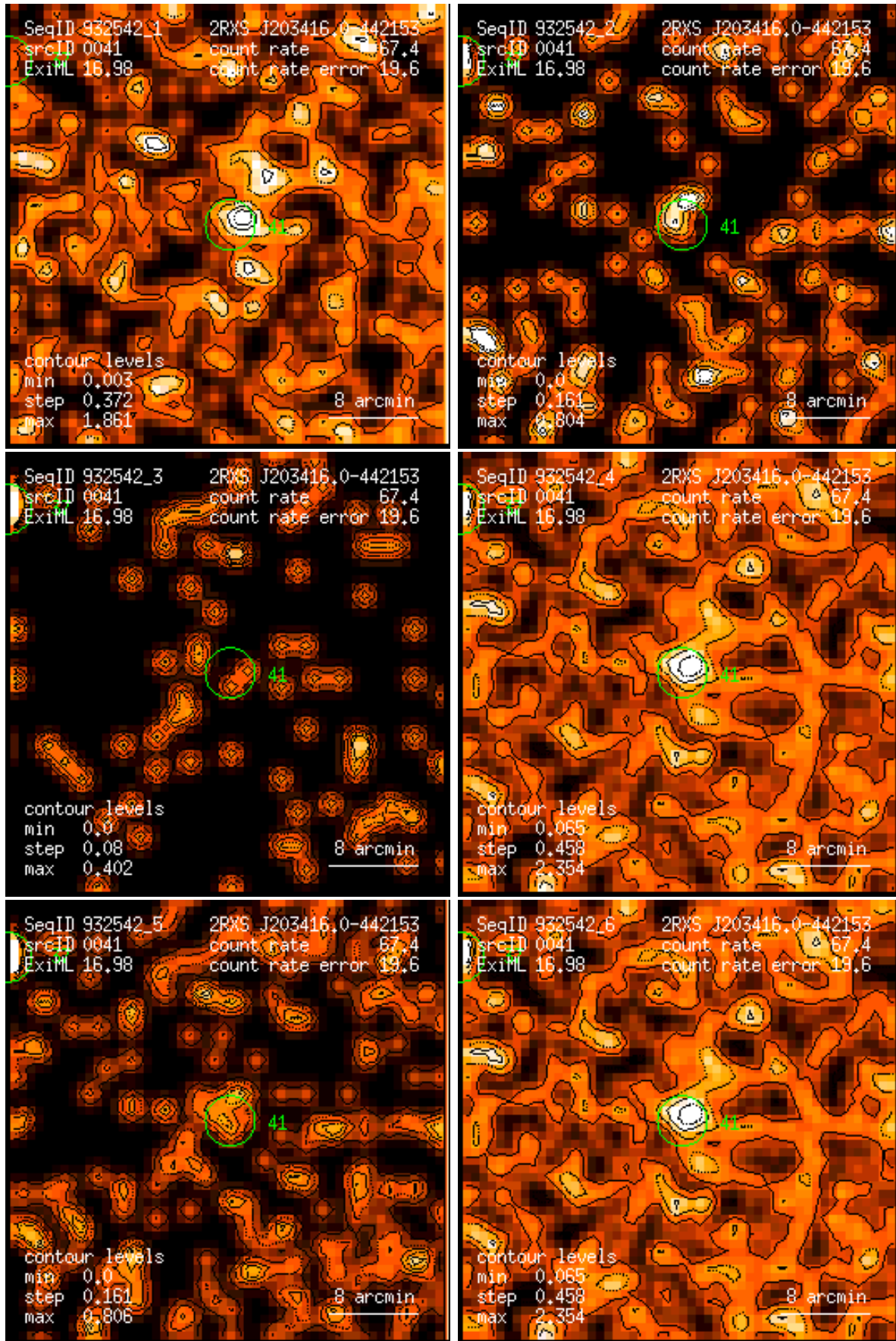
Figure 41: RASS 932542: detection 0041: band rate images, Gaussian filter: (1) PSPC channels 11 – 41, (2) 52 – 90, (3) 91 – 201, (4) 11 – 235, (5) 52 – 201, (6) 11 – 201. Broad band rates in counts/ks. Band rate contour levels in counts/ks/arcmin 2 .
