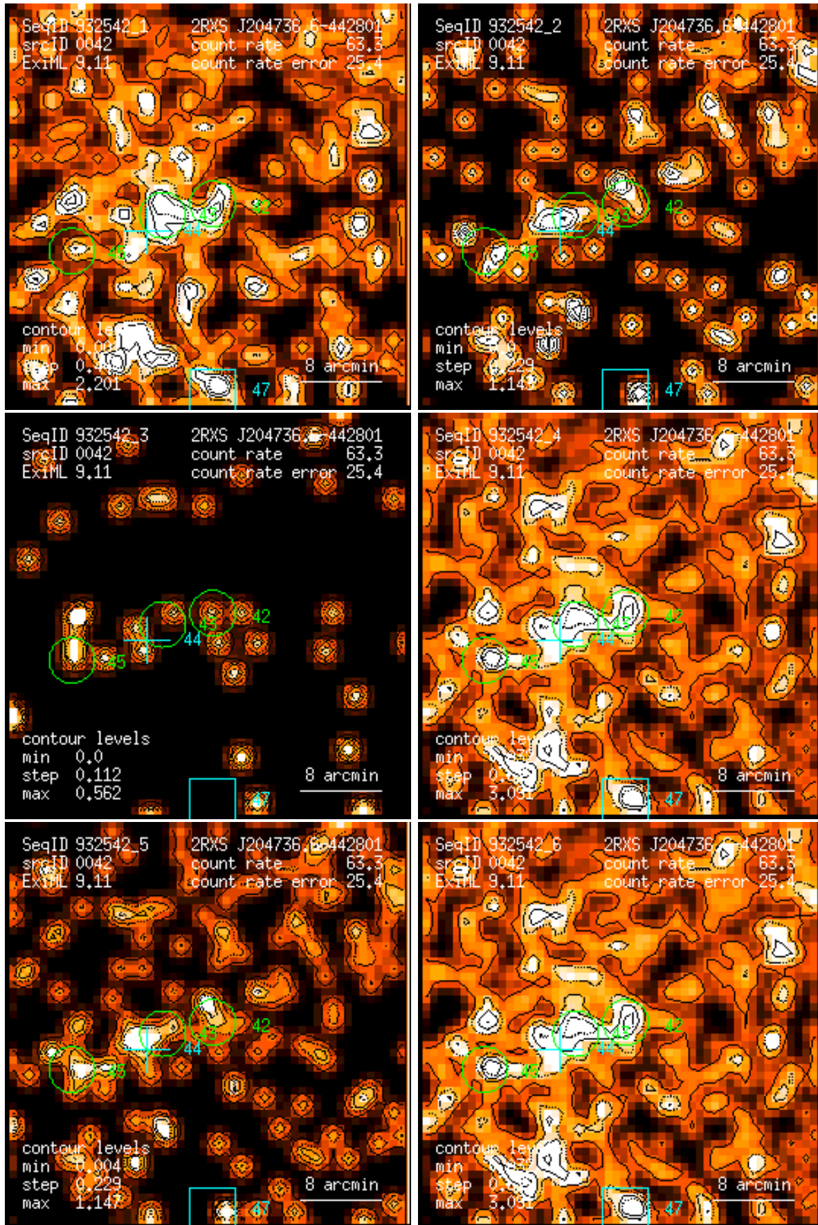
Figure 42: RASS 932542: detection 0042: band rate images, Gaussian filter: (1) PSPC channels 11 – 41, (2) 52 – 90, (3) 91 – 201, (4) 11 – 235, (5) 52 – 201, (6) 11 – 201. Broad band rates in counts/ks. Band rate contour levels in counts/ks/arcmin 2 .
