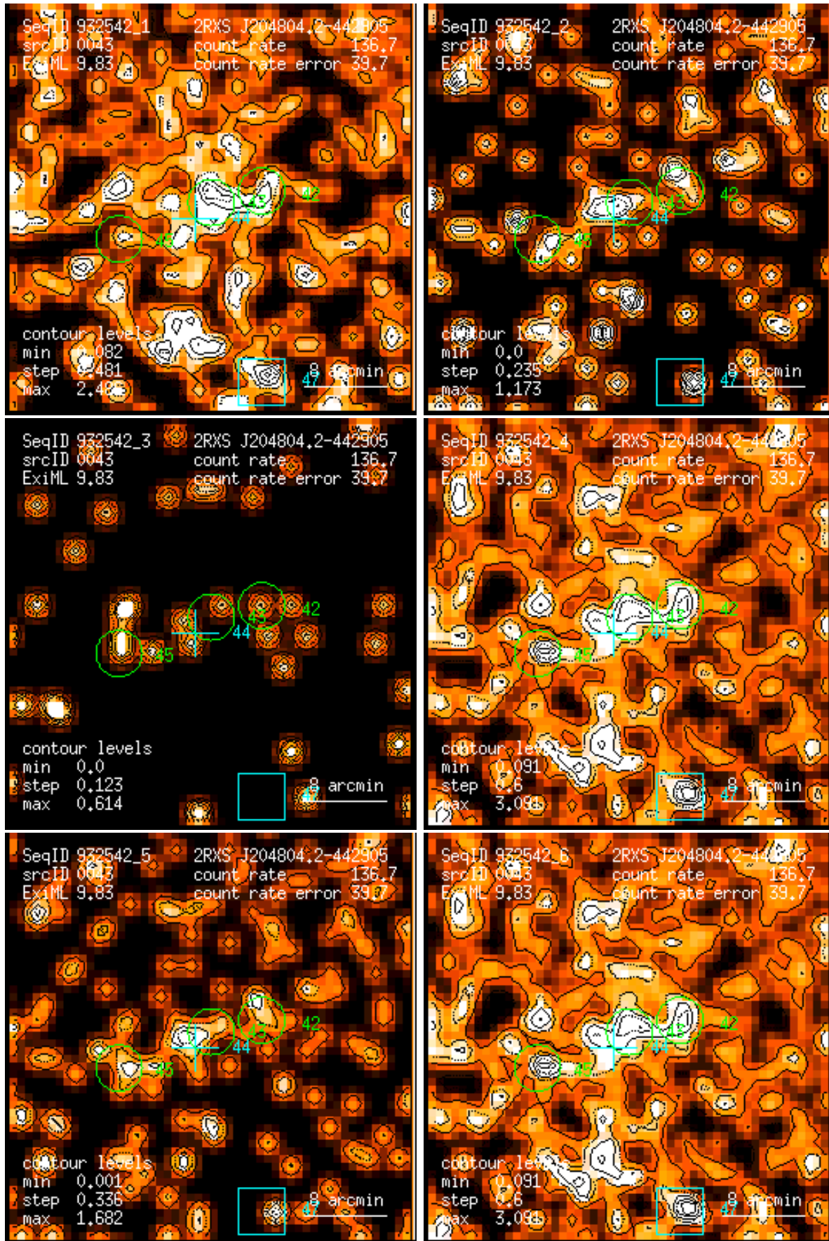
Figure 43: RASS 932542: detection 0043: band rate images, Gaussian filter: (1) PSPC channels 11 – 41, (2) 52 – 90, (3) 91 – 201, (4) 11 – 235, (5) 52 – 201, (6) 11 – 201. Broad band rates in counts/ks. Band rate contour levels in counts/ks/arcmin 2 .
