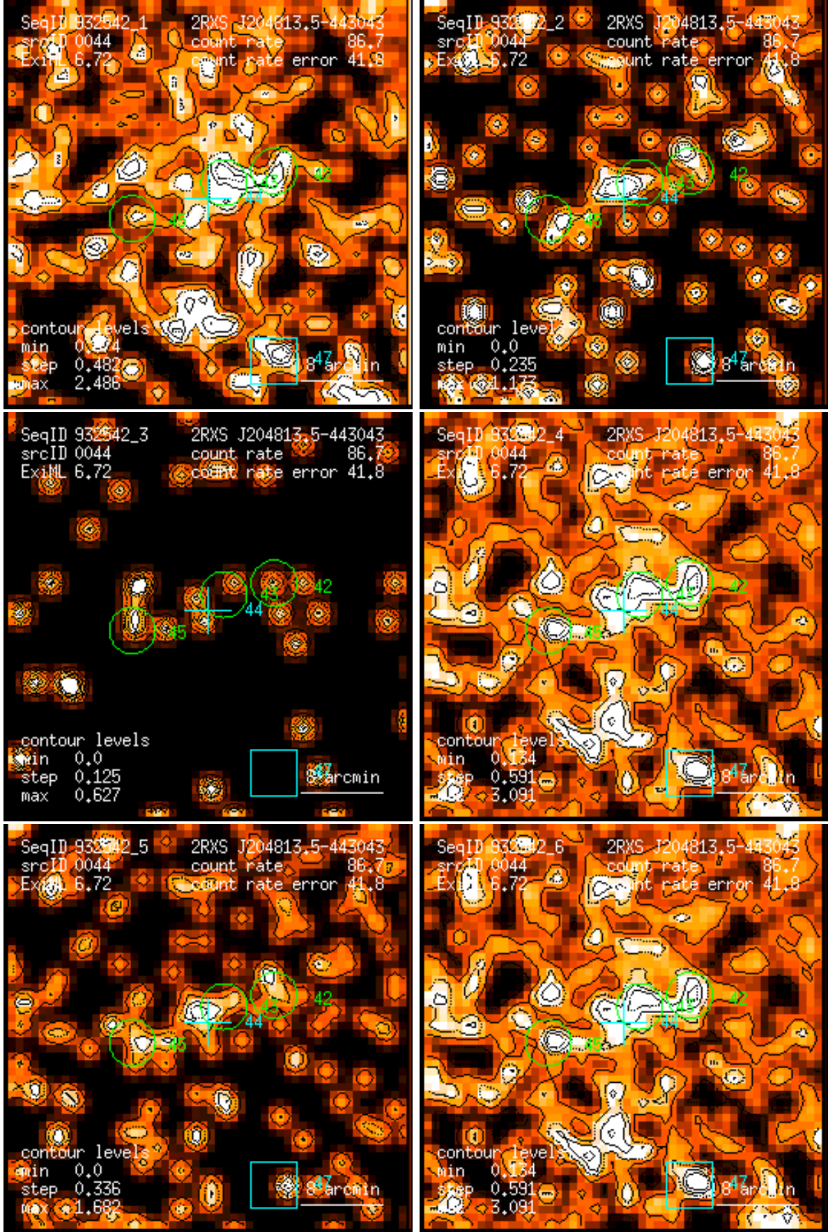
Figure 44: RASS 932542: detection 0044: band rate images, Gaussian filter: (1) PSPC channels 11 – 41, (2) 52 – 90, (3) 91 – 201, (4) 11 – 235, (5) 52 – 201, (6) 11 – 201. Broad band rates in counts/ks. Band rate contour levels in counts/ks/arcmin 2 .
