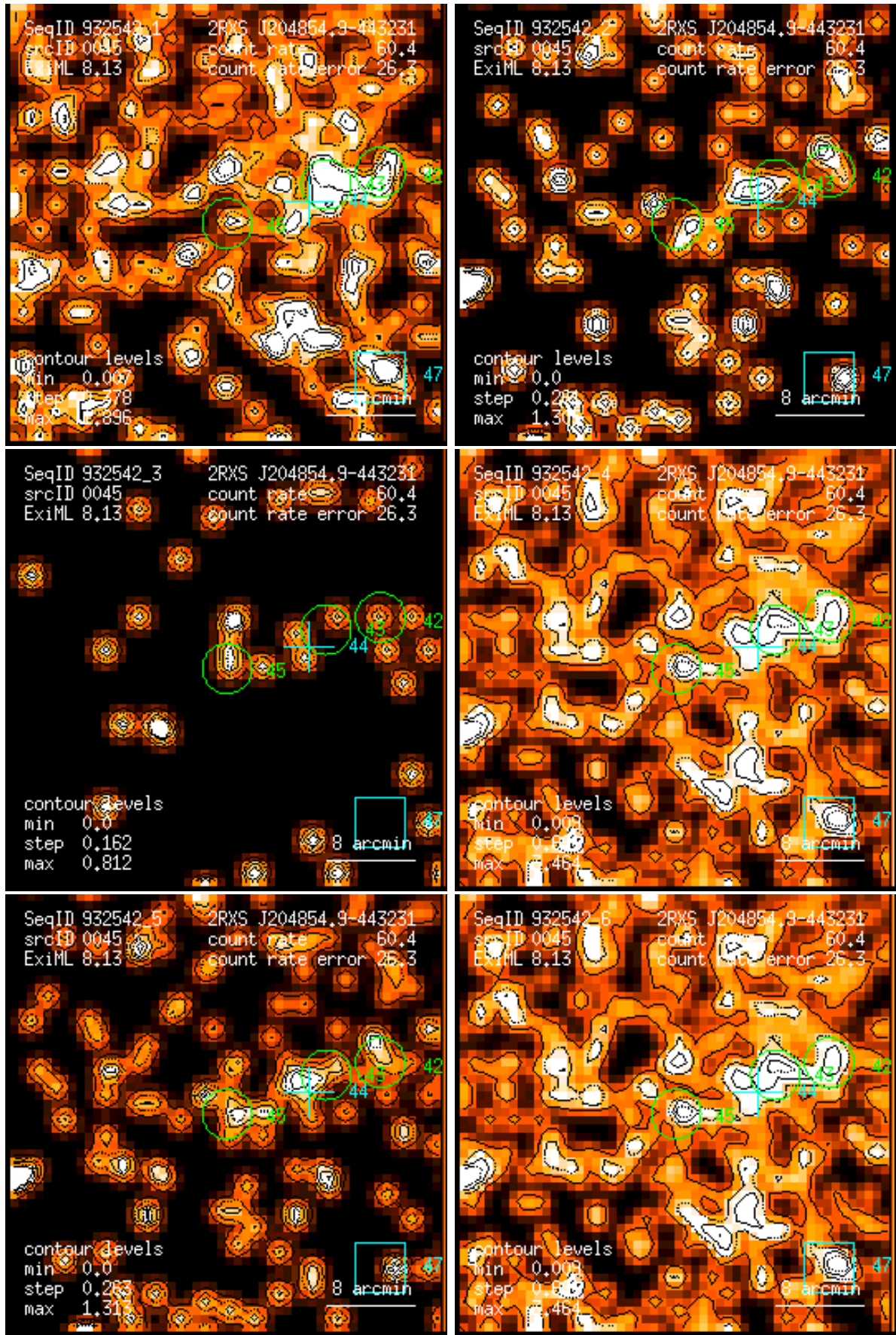
Figure 45: RASS 932542: detection 0045: band rate images, Gaussian filter: (1) PSPC channels 11 – 41, (2) 52 – 90, (3) 91 – 201, (4) 11 – 235, (5) 52 – 201, (6) 11 – 201. Broad band rates in counts/ks. Band rate contour levels in counts/ks/arcmin 2 .
