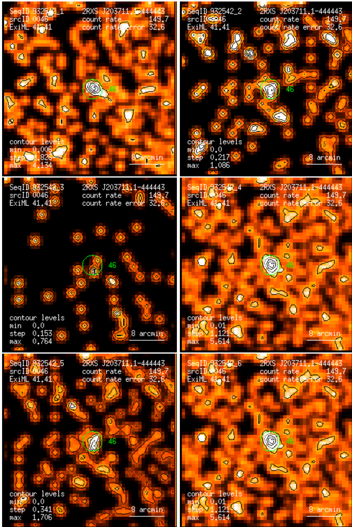
Figure 46: RASS 932542: detection 0046: band rate images, Gaussian filter: (1) PSPC channels 11 – 41, (2) 52 – 90, (3) 91 – 201, (4) 11 – 235, (5) 52 – 201, (6) 11 – 201. Broad band rates in counts/ks. Band rate contour levels in counts/ks/arcmin 2 .
