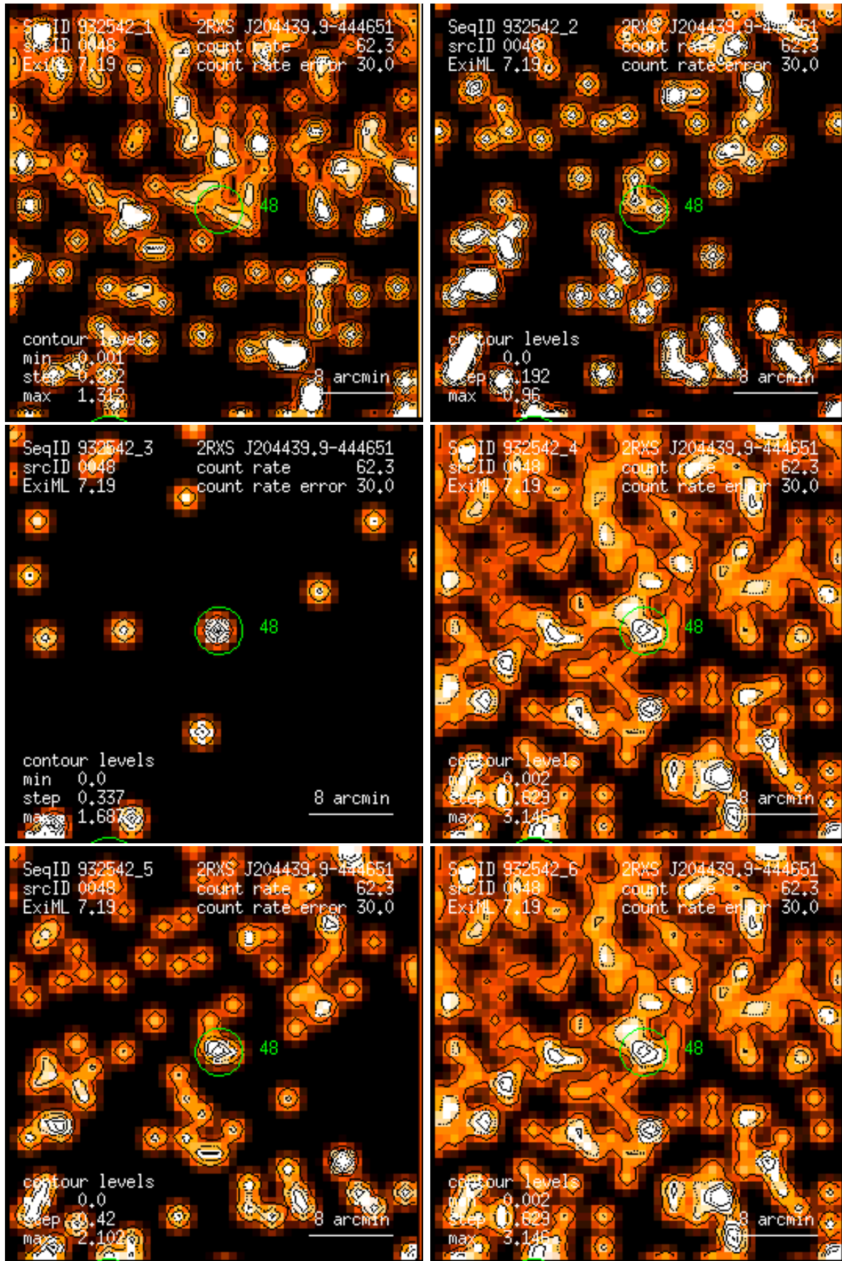
Figure 48: RASS 932542: detection 0048: band rate images, Gaussian filter: (1) PSPC channels 11 – 41, (2) 52 – 90, (3) 91 – 201, (4) 11 – 235, (5) 52 – 201, (6) 11 – 201. Broad band rates in counts/ks. Band rate contour levels in counts/ks/arcmin 2 .
