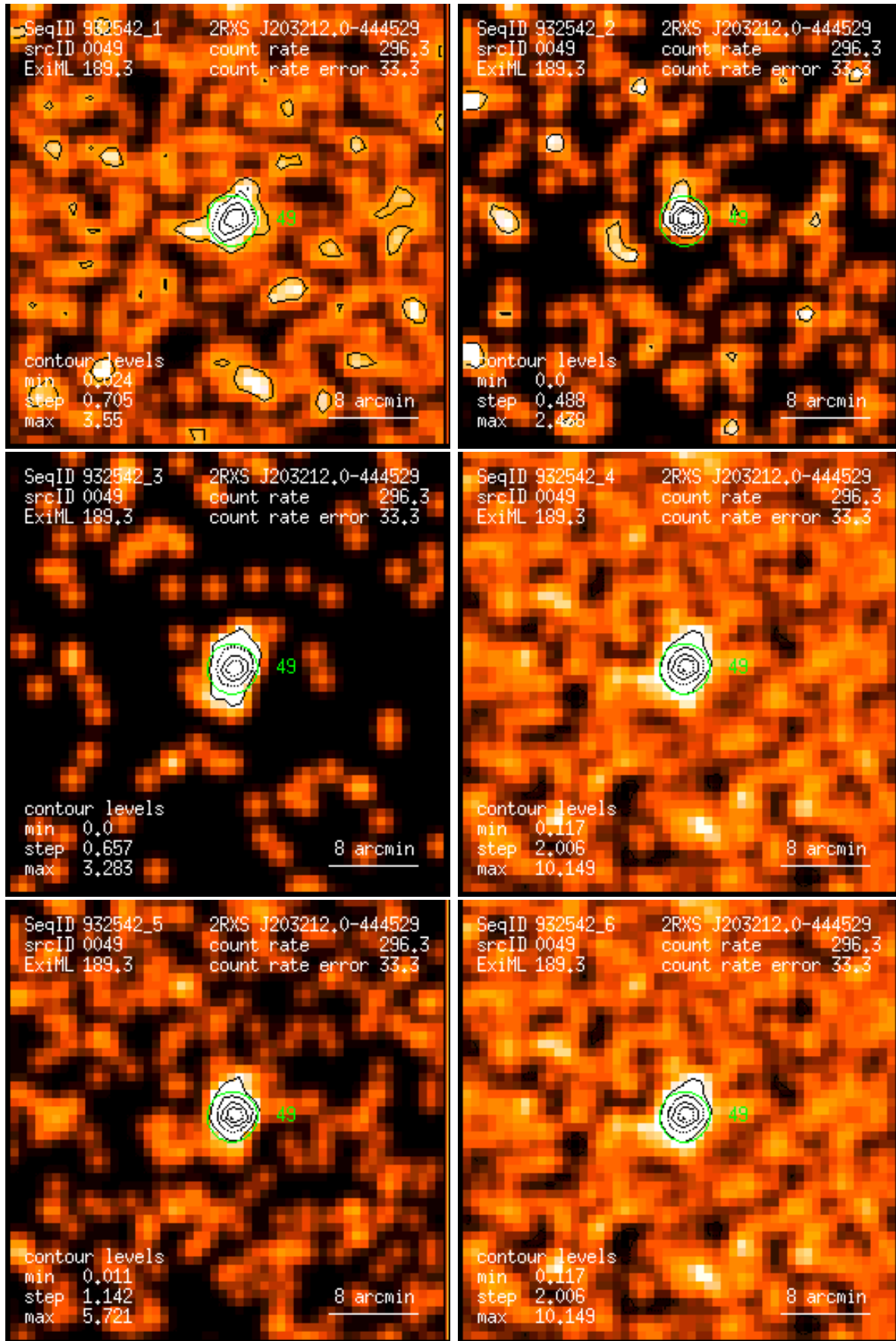
Figure 49: RASS 932542: detection 0049: band rate images, Gaussian filter: (1) PSPC channels 11 – 41, (2) 52 – 90, (3) 91 – 201, (4) 11 – 235, (5) 52 – 201, (6) 11 – 201. Broad band rates in counts/ks. Band rate contour levels in counts/ks/arcmin 2 .
