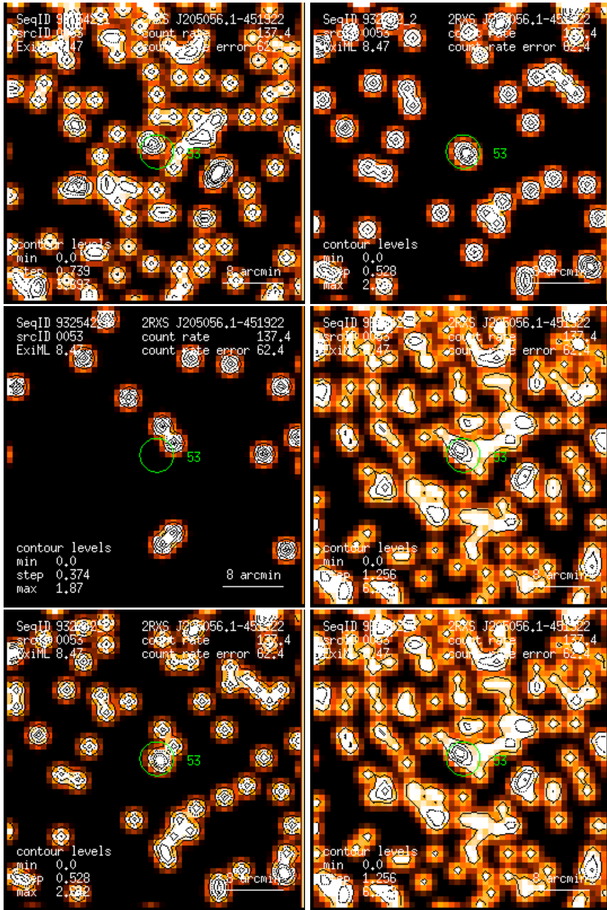
Figure 53: RASS 932542: detection 0053: band rate images, Gaussian filter: (1) PSPC channels 11 – 41, (2) 52 – 90, (3) 91 – 201, (4) 11 – 235, (5) 52 – 201, (6) 11 – 201. Broad band rates in counts/ks. Band rate contour levels in counts/ks/arcmin 2 .
