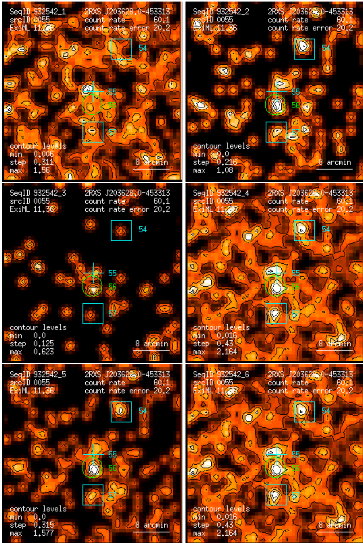
Figure 55: RASS 932542: detection 0055: band rate images, Gaussian filter: (1) PSPC channels 11 – 41, (2) 52 – 90, (3) 91 – 201, (4) 11 – 235, (5) 52 – 201, (6) 11 – 201. Broad band rates in counts/ks. Band rate contour levels in counts/ks/arcmin 2 .
