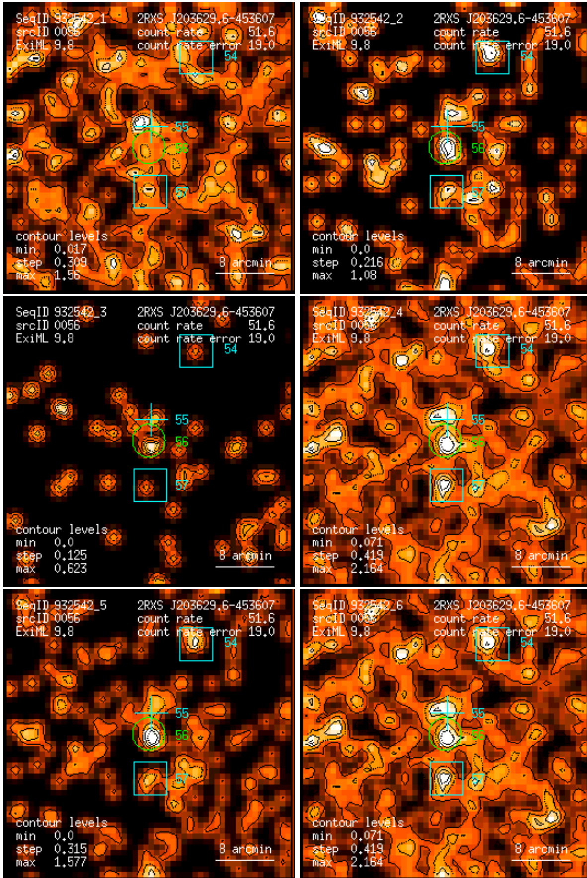
Figure 56: RASS 932542: detection 0056: band rate images, Gaussian filter: (1) PSPC channels 11 – 41, (2) 52 – 90, (3) 91 – 201, (4) 11 – 235, (5) 52 – 201, (6) 11 – 201. Broad band rates in counts/ks. Band rate contour levels in counts/ks/arcmin 2 .
