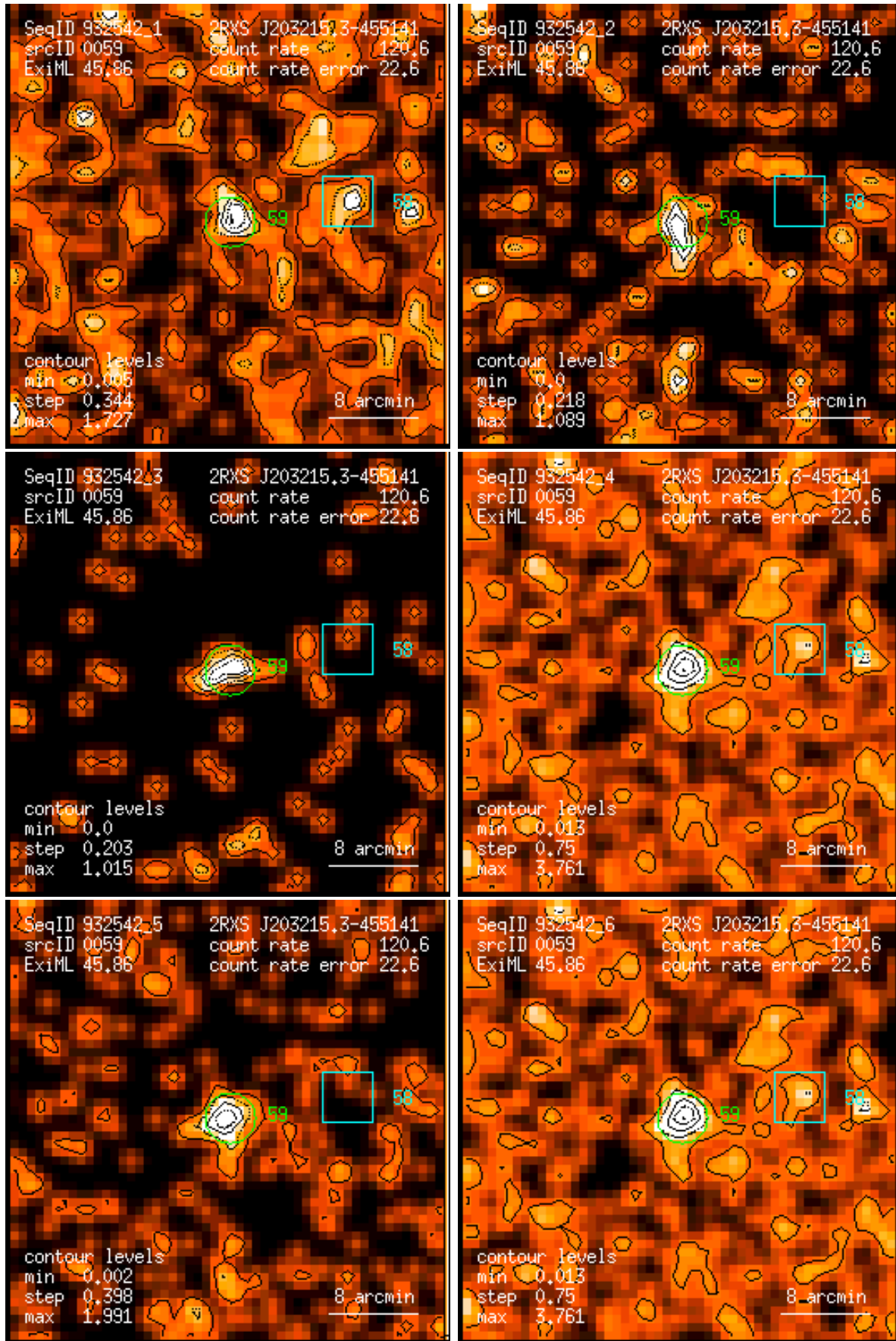
Figure 59: RASS 932542: detection 0059: band rate images, Gaussian filter: (1) PSPC channels 11 – 41, (2) 52 – 90, (3) 91 – 201, (4) 11 – 235, (5) 52 – 201, (6) 11 – 201. Broad band rates in counts/ks. Band rate contour levels in counts/ks/arcmin 2 .
