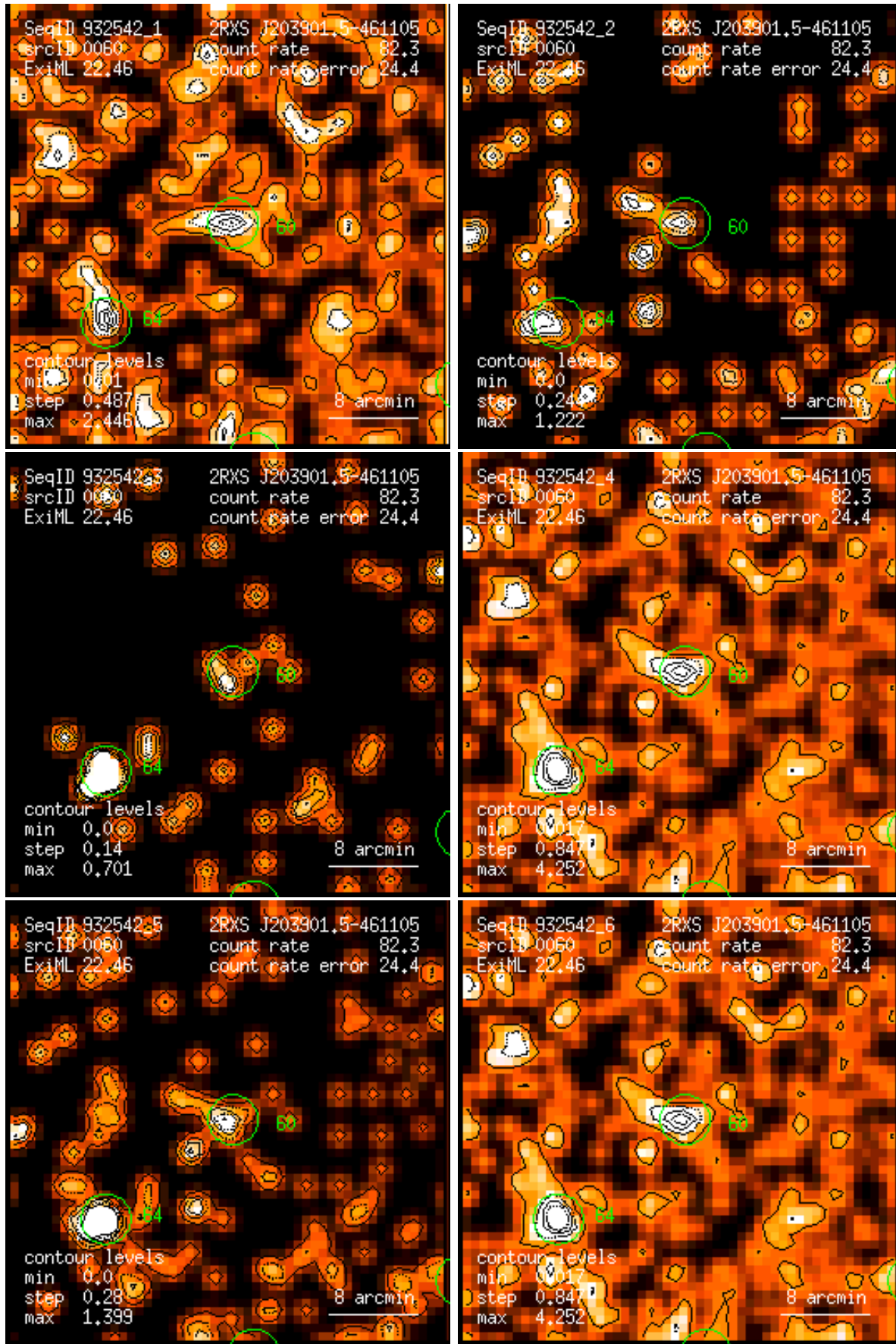
Figure 60: RASS 932542: detection 0060: band rate images, Gaussian filter: (1) PSPC channels 11 – 41, (2) 52 – 90, (3) 91 – 201, (4) 11 – 235, (5) 52 – 201, (6) 11 – 201. Broad band rates in counts/ks. Band rate contour levels in counts/ks/arcmin 2 .
