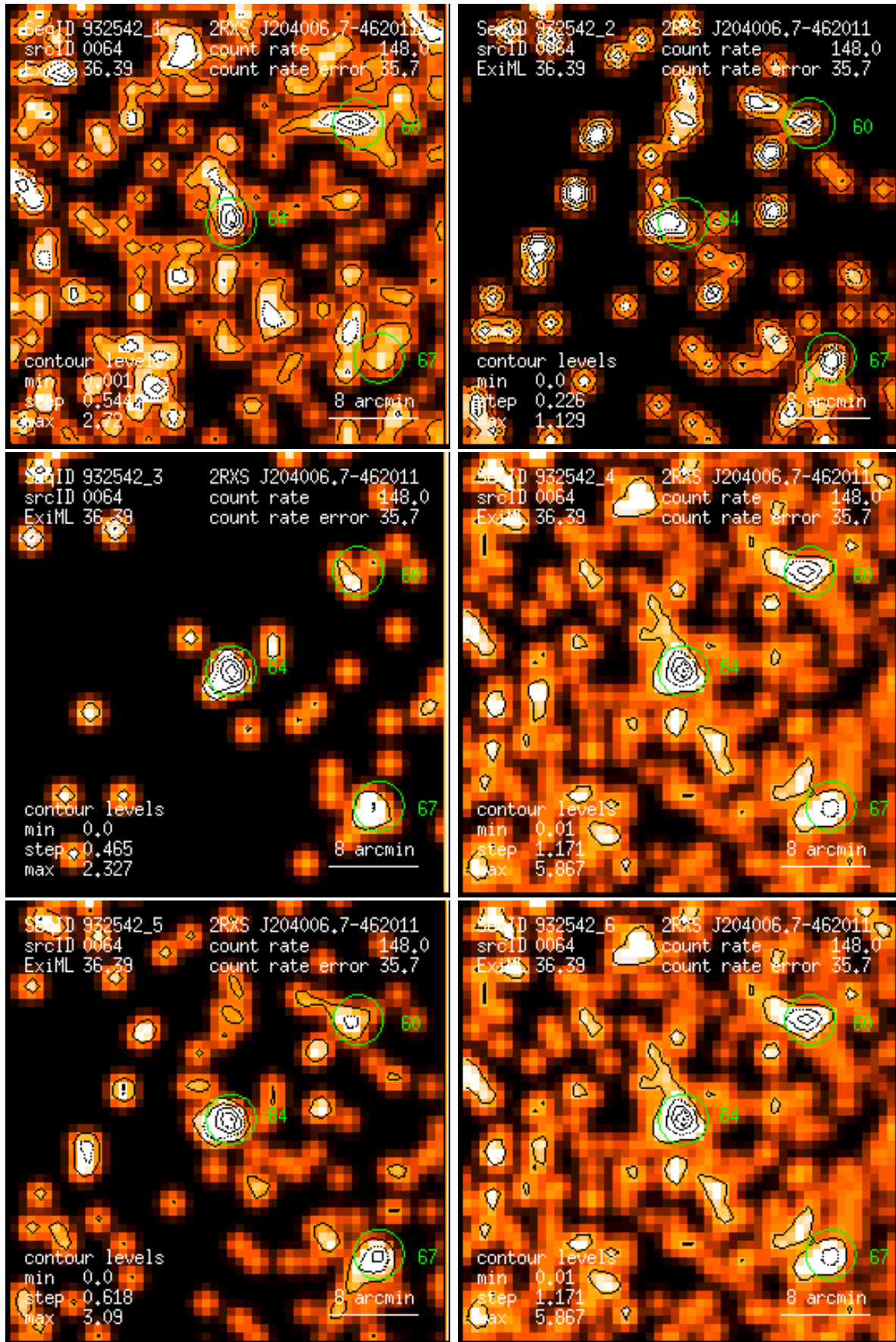
Figure 64: RASS 932542: detection 0064: band rate images, Gaussian filter: (1) PSPC channels 11 – 41, (2) 52 – 90, (3) 91 – 201, (4) 11 – 235, (5) 52 – 201, (6) 11 – 201. Broad band rates in counts/ks. Band rate contour levels in counts/ks/arcmin 2 .
