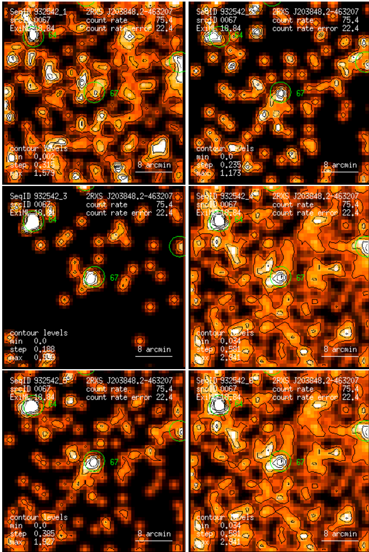
Figure 67: RASS 932542: detection 0067: band rate images, Gaussian filter: (1) PSPC channels 11 – 41, (2) 52 – 90, (3) 91 – 201, (4) 11 – 235, (5) 52 – 201, (6) 11 – 201. Broad band rates in counts/ks. Band rate contour levels in counts/ks/arcmin 2 .
