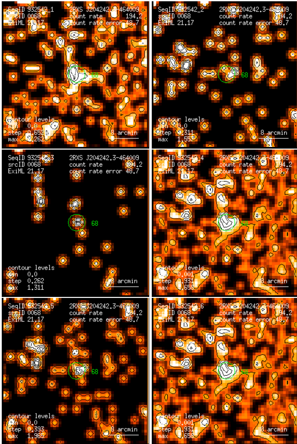
Figure 68: RASS 932542: detection 0068: band rate images, Gaussian filter: (1) PSPC channels 11 – 41, (2) 52 – 90, (3) 91 – 201, (4) 11 – 235, (5) 52 – 201, (6) 11 – 201. Broad band rates in counts/ks. Band rate contour levels in counts/ks/arcmin 2 .
