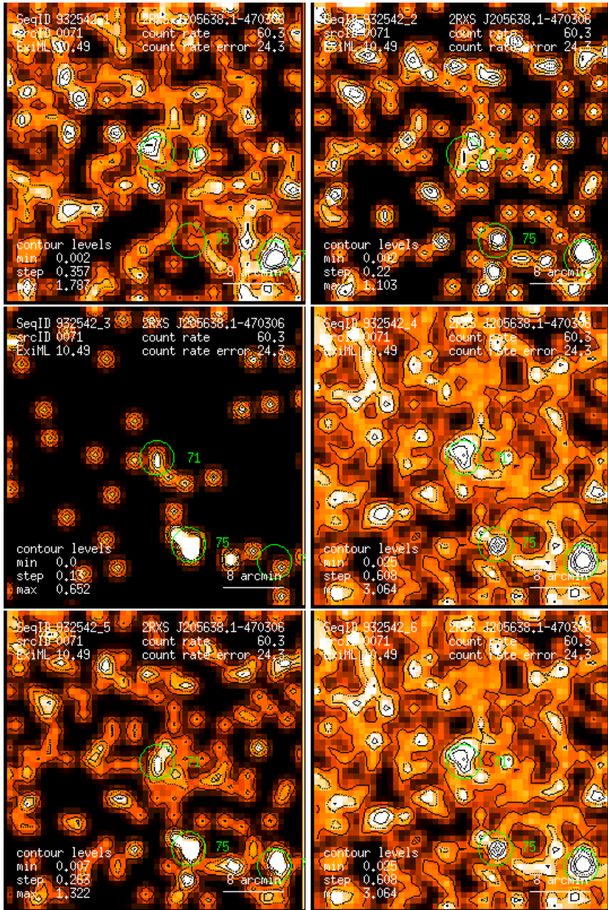
Figure 71: RASS 932542: detection 0071: band rate images, Gaussian filter: (1) PSPC channels 11 – 41, (2) 52 – 90, (3) 91 – 201, (4) 11 – 235, (5) 52 – 201, (6) 11 – 201. Broad band rates in counts/ks. Band rate contour levels in counts/ks/arcmin 2 .
