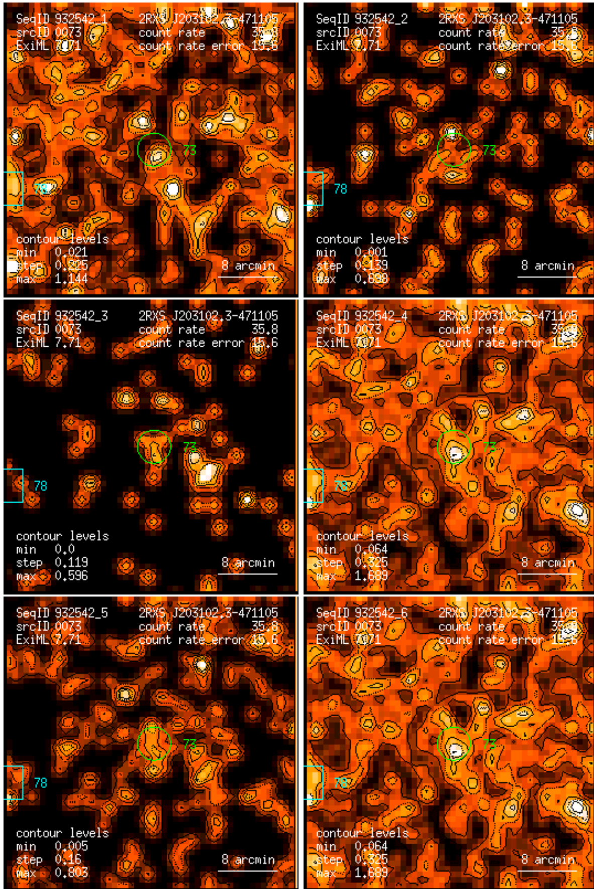
Figure 73: RASS 932542: detection 0073: band rate images, Gaussian filter: (1) PSPC channels 11 – 41, (2) 52 – 90, (3) 91 – 201, (4) 11 – 235, (5) 52 – 201, (6) 11 – 201. Broad band rates in counts/ks. Band rate contour levels in counts/ks/arcmin 2 .
