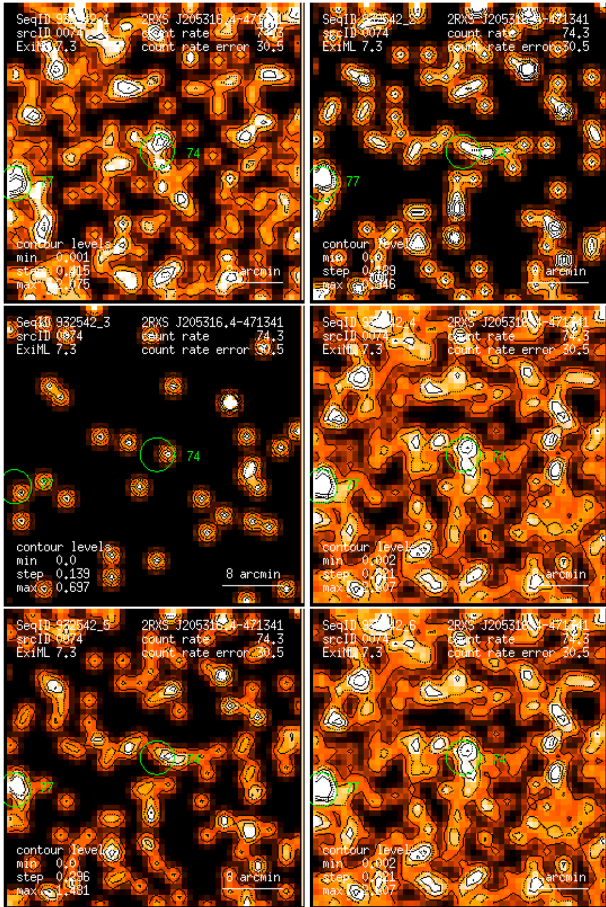
Figure 74: RASS 932542: detection 0074: band rate images, Gaussian filter: (1) PSPC channels 11 – 41, (2) 52 – 90, (3) 91 – 201, (4) 11 – 235, (5) 52 – 201, (6) 11 – 201. Broad band rates in counts/ks. Band rate contour levels in counts/ks/arcmin 2 .
