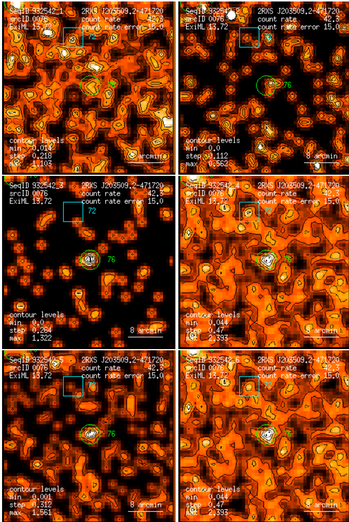
Figure 76: RASS 932542: detection 0076: band rate images, Gaussian filter: (1) PSPC channels 11 – 41, (2) 52 – 90, (3) 91 – 201, (4) 11 – 235, (5) 52 – 201, (6) 11 – 201. Broad band rates in counts/ks. Band rate contour levels in counts/ks/arcmin 2 .
