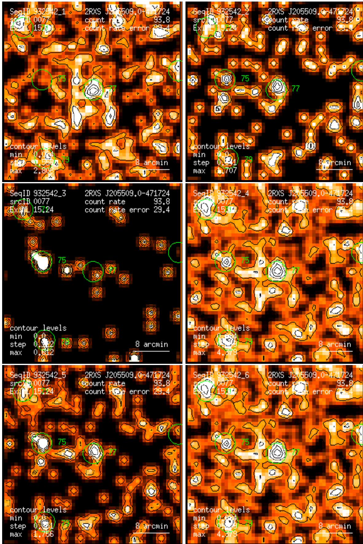
Figure 77: RASS 932542: detection 0077: band rate images, Gaussian filter: (1) PSPC channels 11 – 41, (2) 52 – 90, (3) 91 – 201, (4) 11 – 235, (5) 52 – 201, (6) 11 – 201. Broad band rates in counts/ks. Band rate contour levels in counts/ks/arcmin 2 .
