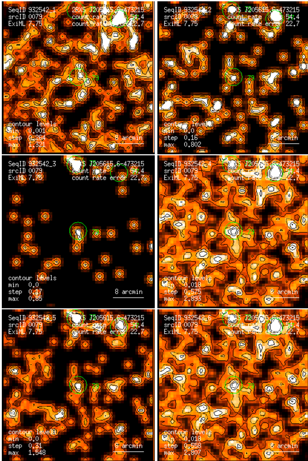
Figure 79: RASS 932542: detection 0079: band rate images, Gaussian filter: (1) PSPC channels 11 – 41, (2) 52 – 90, (3) 91 – 201, (4) 11 – 235, (5) 52 – 201, (6) 11 – 201. Broad band rates in counts/ks. Band rate contour levels in counts/ks/arcmin 2 .
