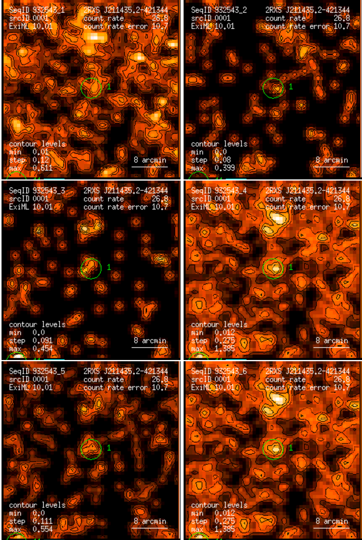
Figure 1: RASS 932543: detection 0001: band rate images, Gaussian filter: (1) PSPC channels 11 – 41, (2) 52 – 90, (3) 91 – 201, (4) 11 – 235, (5) 52 – 201, (6) 11 – 201. Broad band rates in counts/ks. Band rate contour levels in counts/ks/arcmin 2 .
