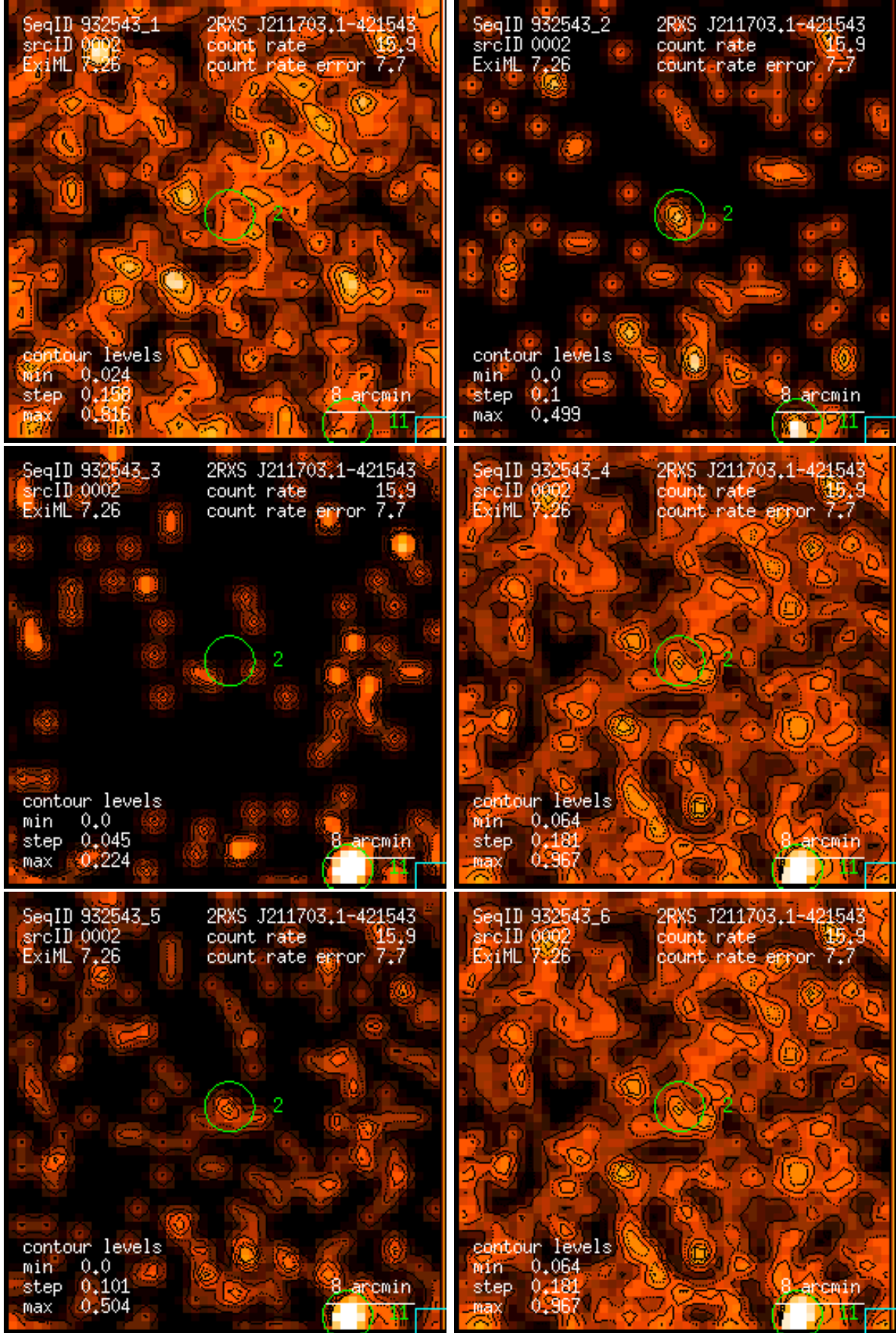
Figure 2: RASS 932543: detection 0002: band rate images, Gaussian filter: (1) PSPC channels 11 – 41, (2) 52 – 90, (3) 91 – 201, (4) 11 – 235, (5) 52 – 201, (6) 11 – 201. Broad band rates in counts/ks. Band rate contour levels in counts/ks/arcmin 2 .
