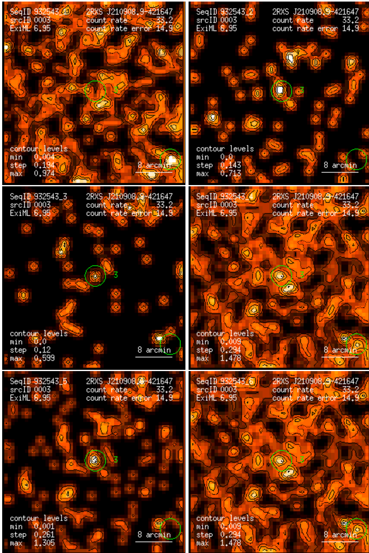
Figure 3: RASS 932543: detection 0003: band rate images, Gaussian filter: (1) PSPC channels 11 – 41, (2) 52 – 90, (3) 91 – 201, (4) 11 – 235, (5) 52 – 201, (6) 11 – 201. Broad band rates in counts/ks. Band rate contour levels in counts/ks/arcmin 2 .
