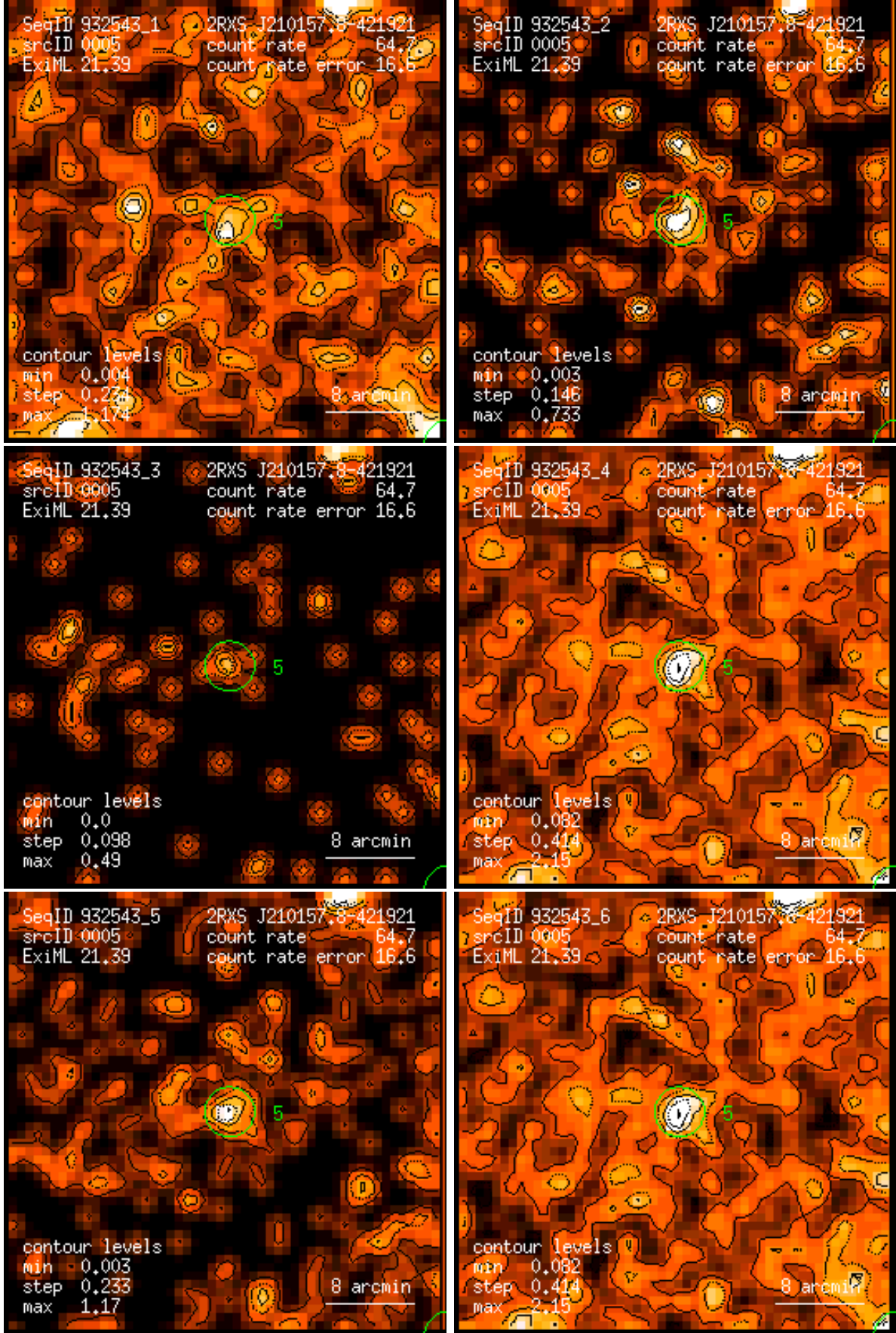
Figure 5: RASS 932543: detection 0005: band rate images, Gaussian filter: (1) PSPC channels 11 – 41, (2) 52 – 90, (3) 91 – 201, (4) 11 – 235, (5) 52 – 201, (6) 11 – 201. Broad band rates in counts/ks. Band rate contour levels in counts/ks/arcmin 2 .
