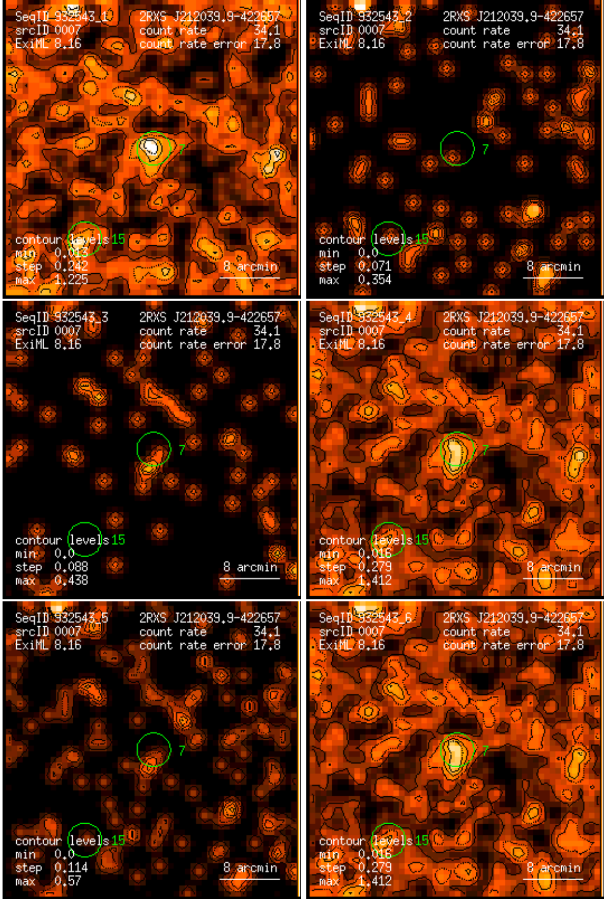
Figure 7: RASS 932543: detection 0007: band rate images, Gaussian filter: (1) PSPC channels 11 – 41, (2) 52 – 90, (3) 91 – 201, (4) 11 – 235, (5) 52 – 201, (6) 11 – 201. Broad band rates in counts/ks. Band rate contour levels in counts/ks/arcmin 2 .
