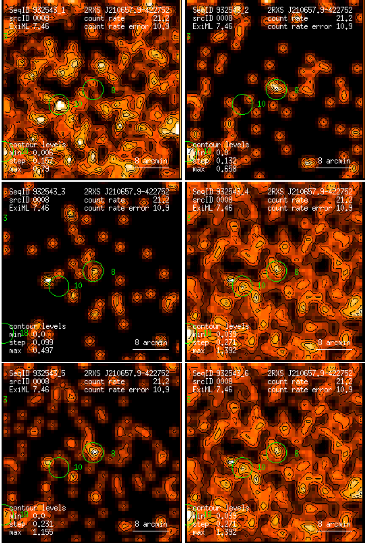
Figure 8: RASS 932543: detection 0008: band rate images, Gaussian filter: (1) PSPC channels 11 – 41, (2) 52 – 90, (3) 91 – 201, (4) 11 – 235, (5) 52 – 201, (6) 11 – 201. Broad band rates in counts/ks. Band rate contour levels in counts/ks/arcmin 2 .
