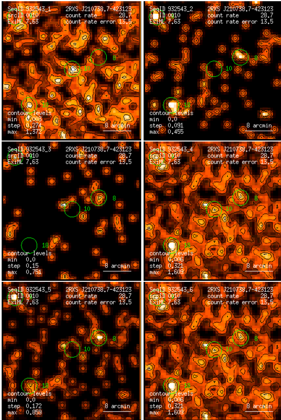
Figure 10: RASS 932543: detection 0010: band rate images, Gaussian filter: (1) PSPC channels 11 – 41, (2) 52 – 90, (3) 91 – 201, (4) 11 – 235, (5) 52 – 201, (6) 11 – 201. Broad band rates in counts/ks. Band rate contour levels in counts/ks/arcmin 2 .
