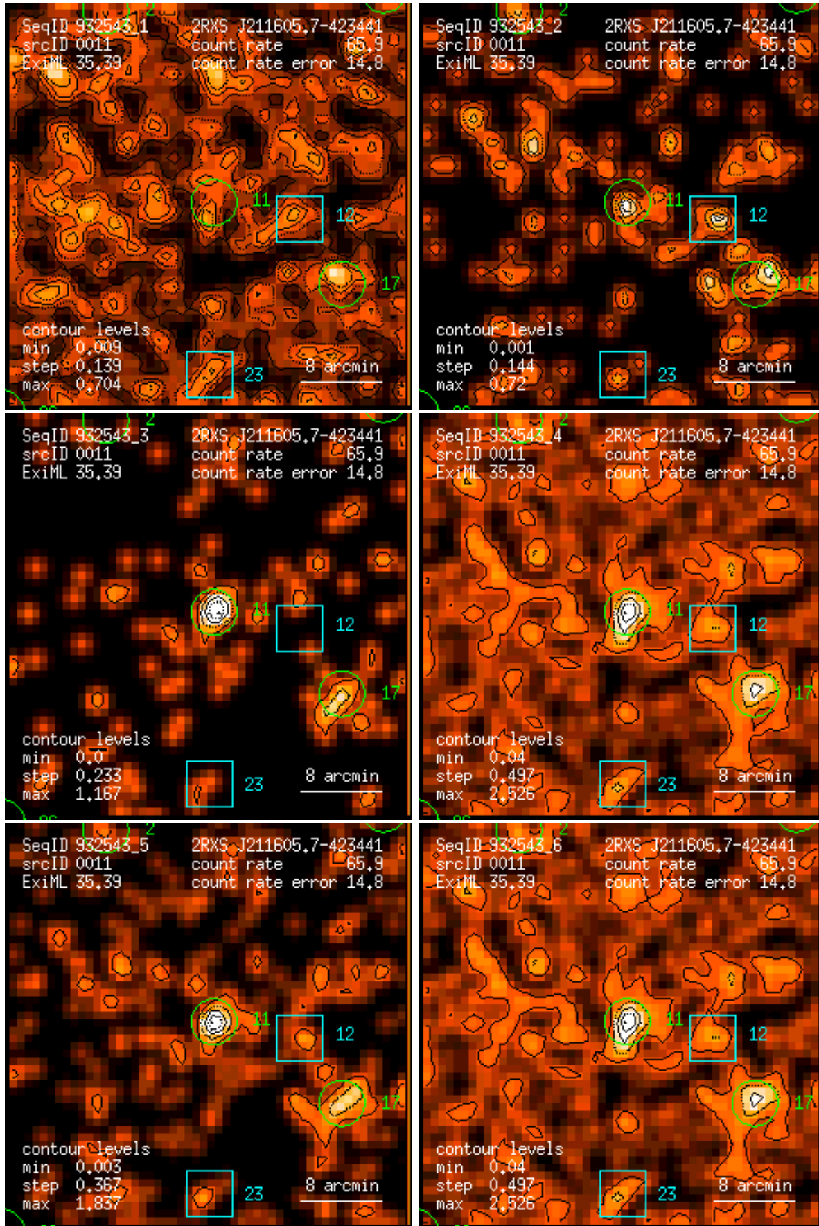
Figure 11: RASS 932543: detection 0011: band rate images, Gaussian filter: (1) PSPC channels 11 – 41, (2) 52 – 90, (3) 91 – 201, (4) 11 – 235, (5) 52 – 201, (6) 11 – 201. Broad band rates in counts/ks. Band rate contour levels in counts/ks/arcmin 2 .
